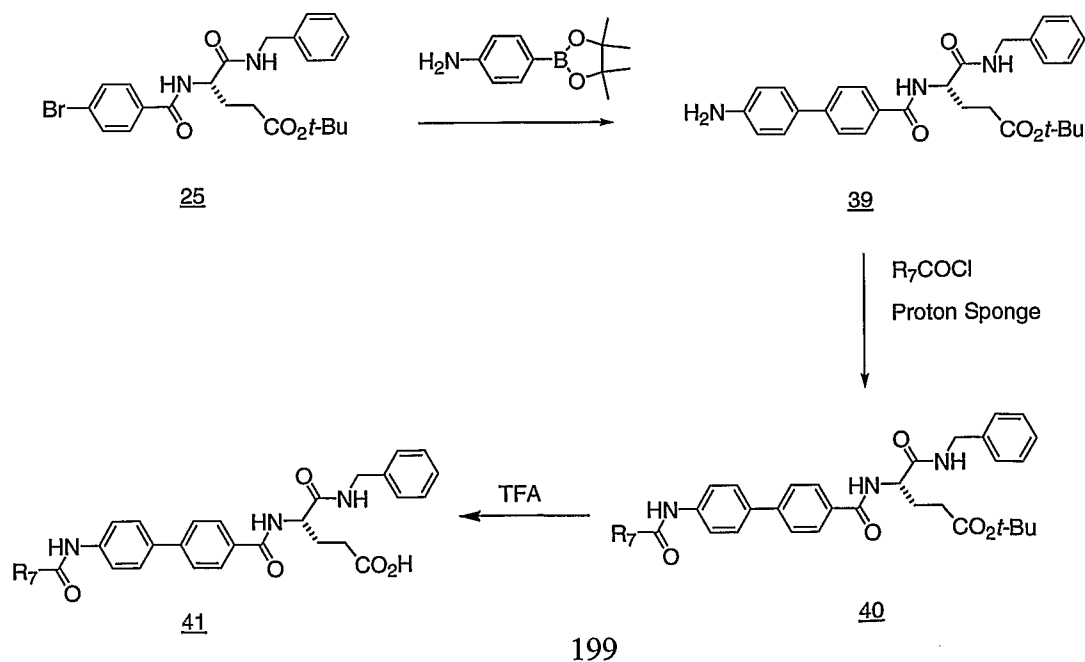
Scheme 13
