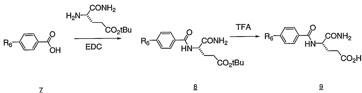
Scheme 3
