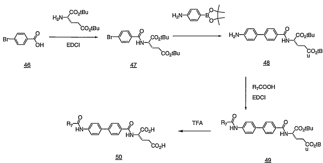
Scheme 15
