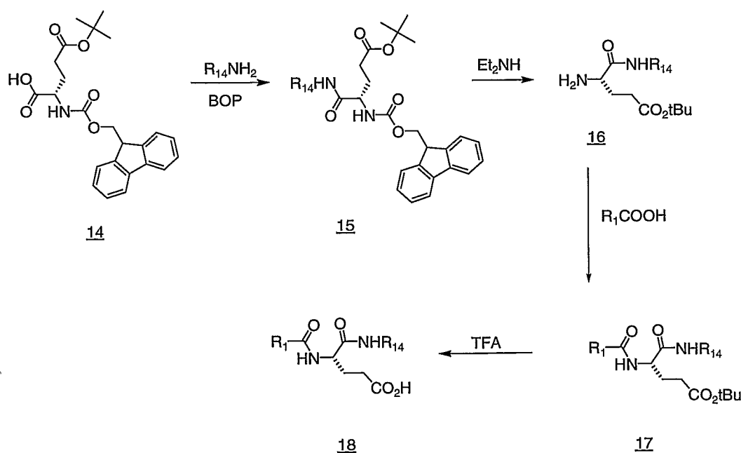
Scheme 7
