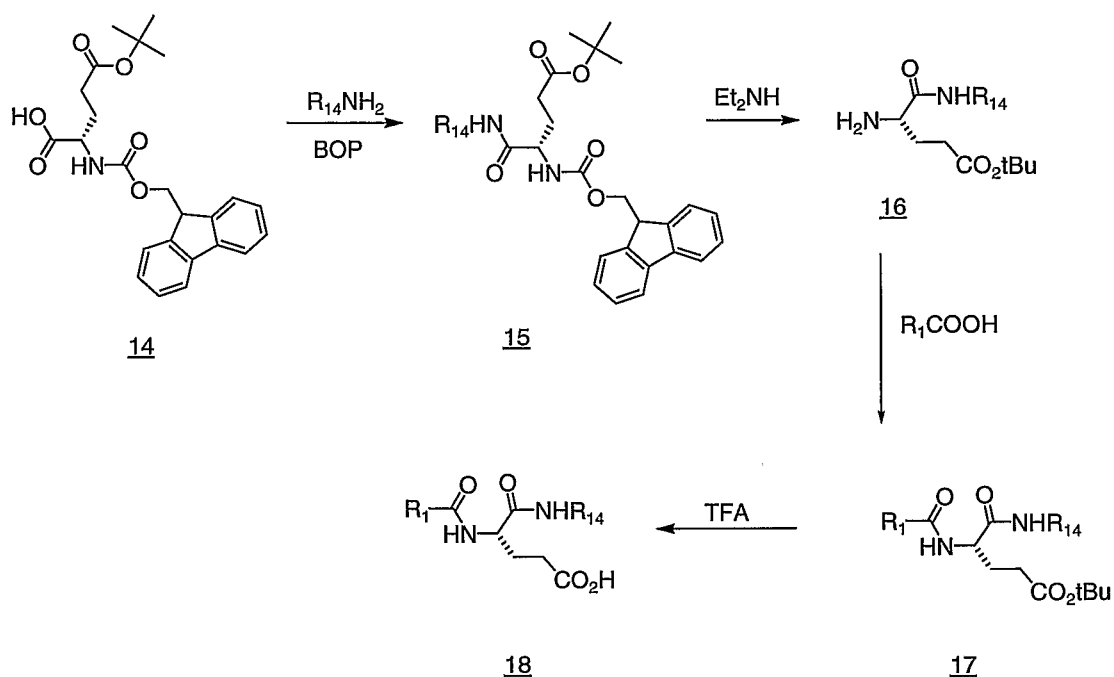
Scheme 7
