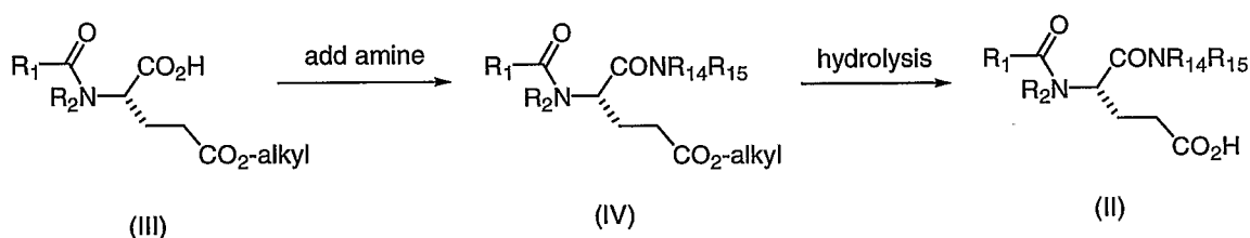
Scheme 4
