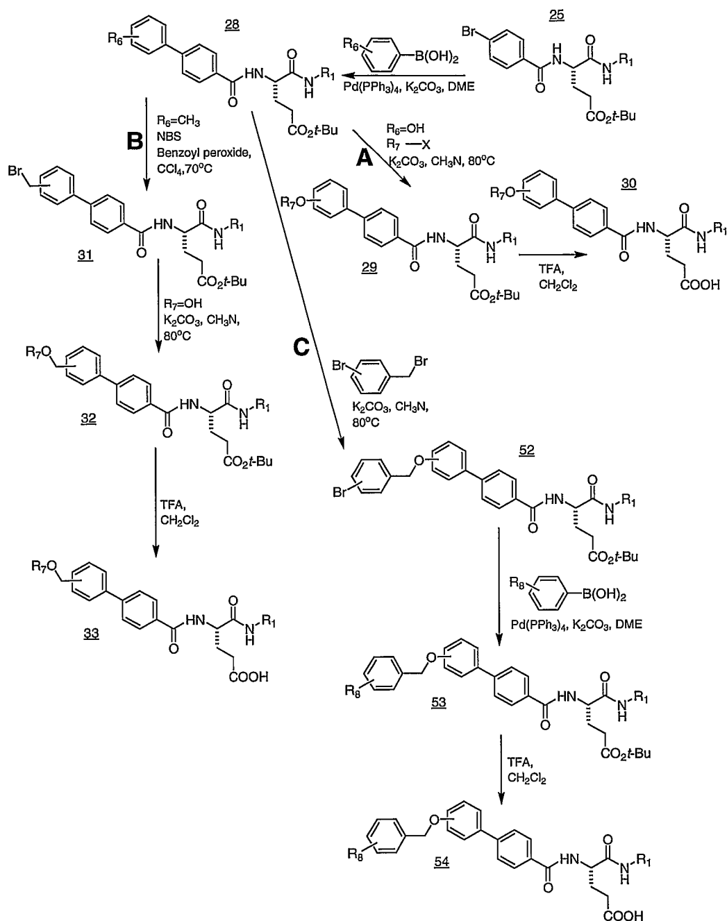
Scheme 10
