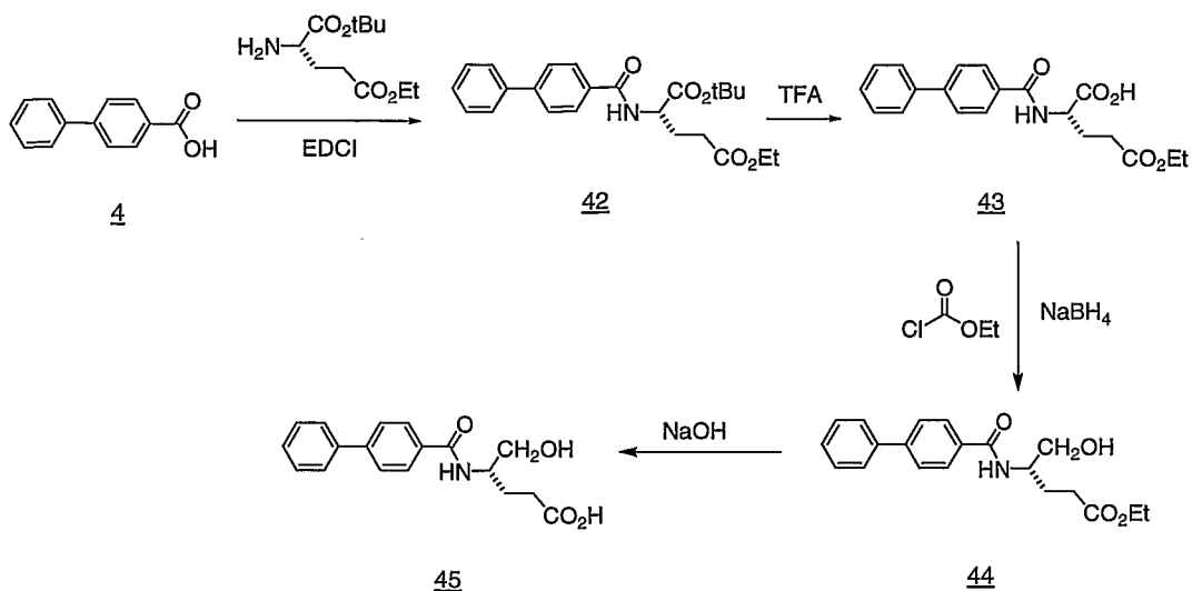
Scheme 14
