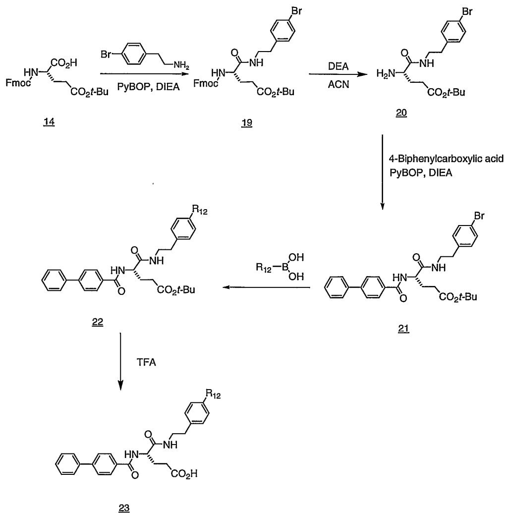
Scheme 8
