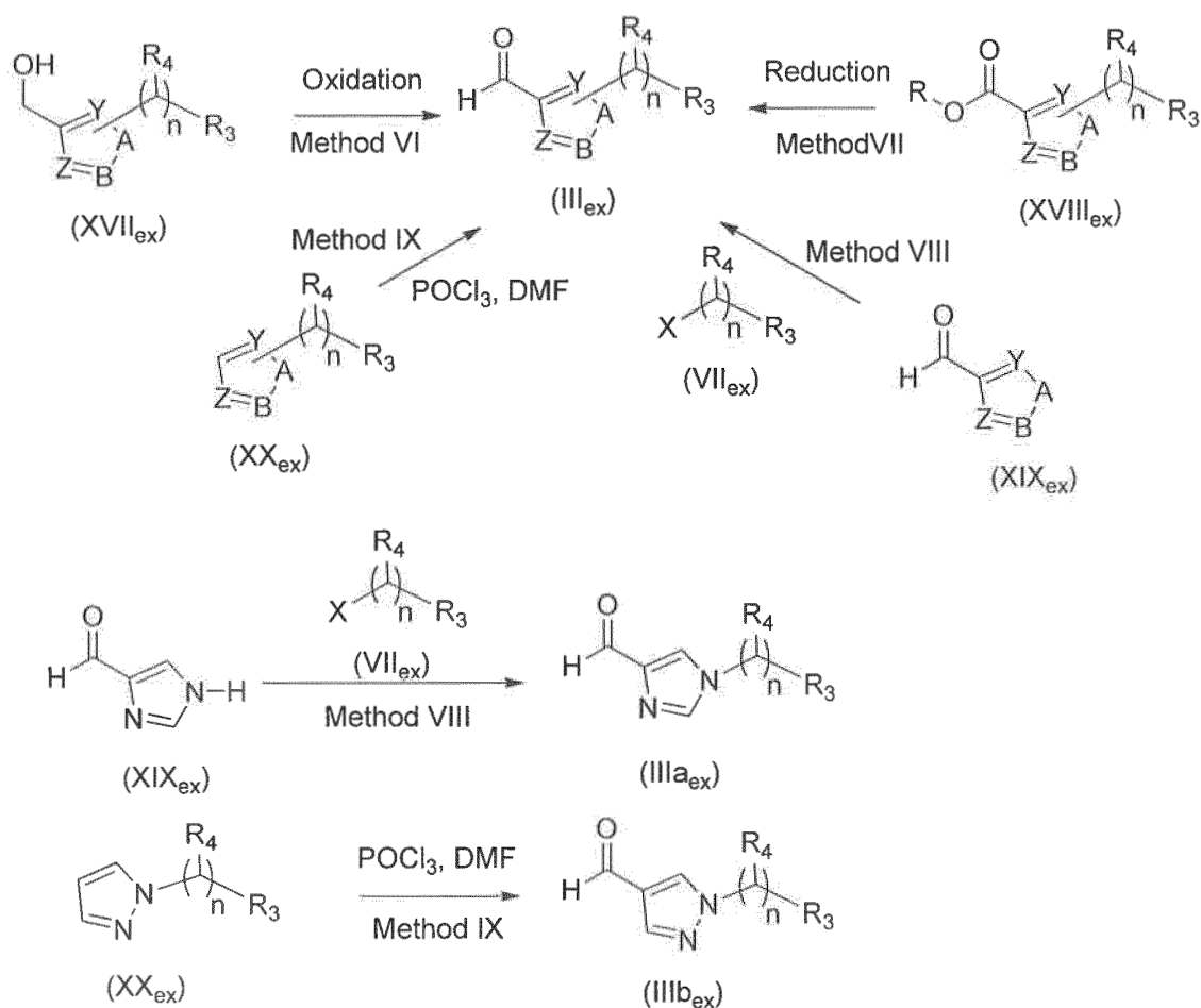
Scheme 6
