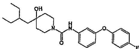
Comparative compound B
