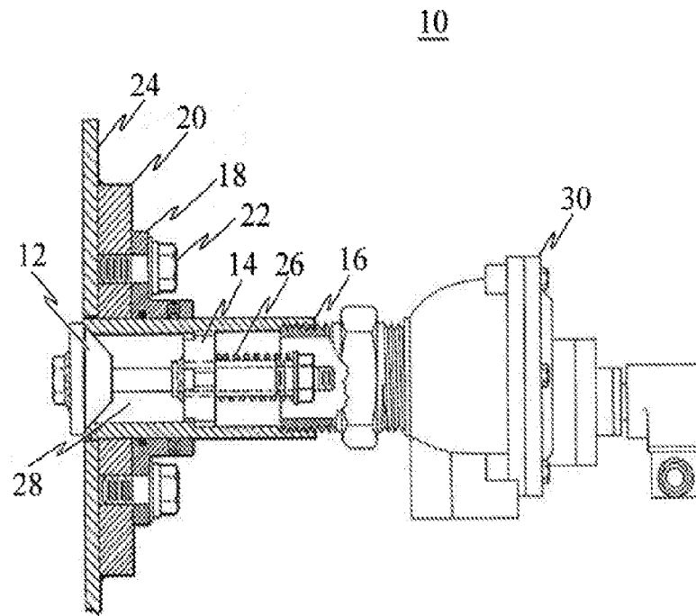
FIG. 1 (PRIOR ART)
