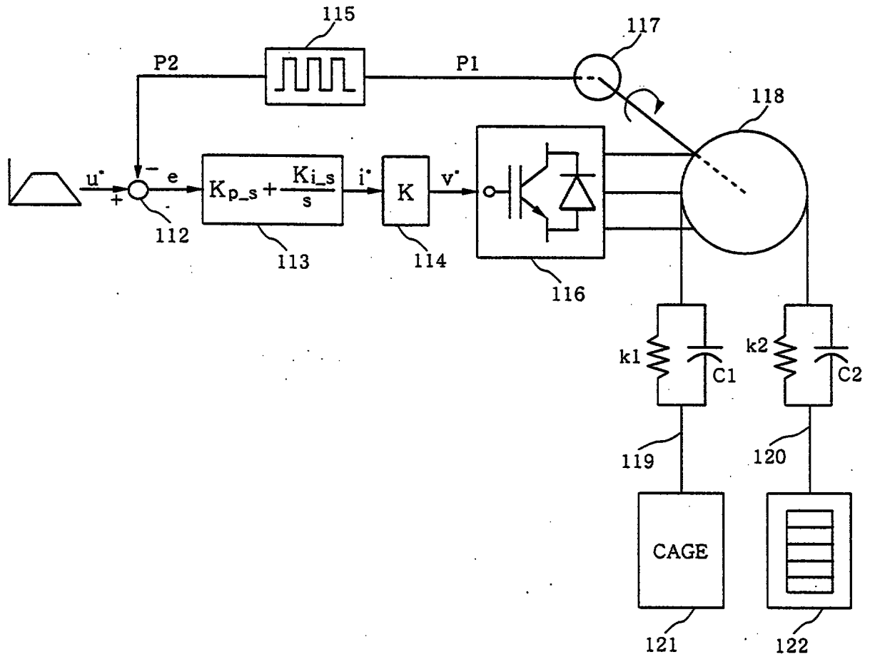
FIG.1 CONVENTIONAL ART
