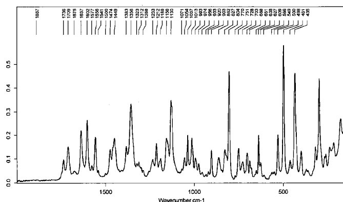
Fig. 1 : FT-Raman spectrum of Formula (1)
