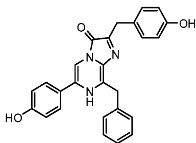
coelenterazine
