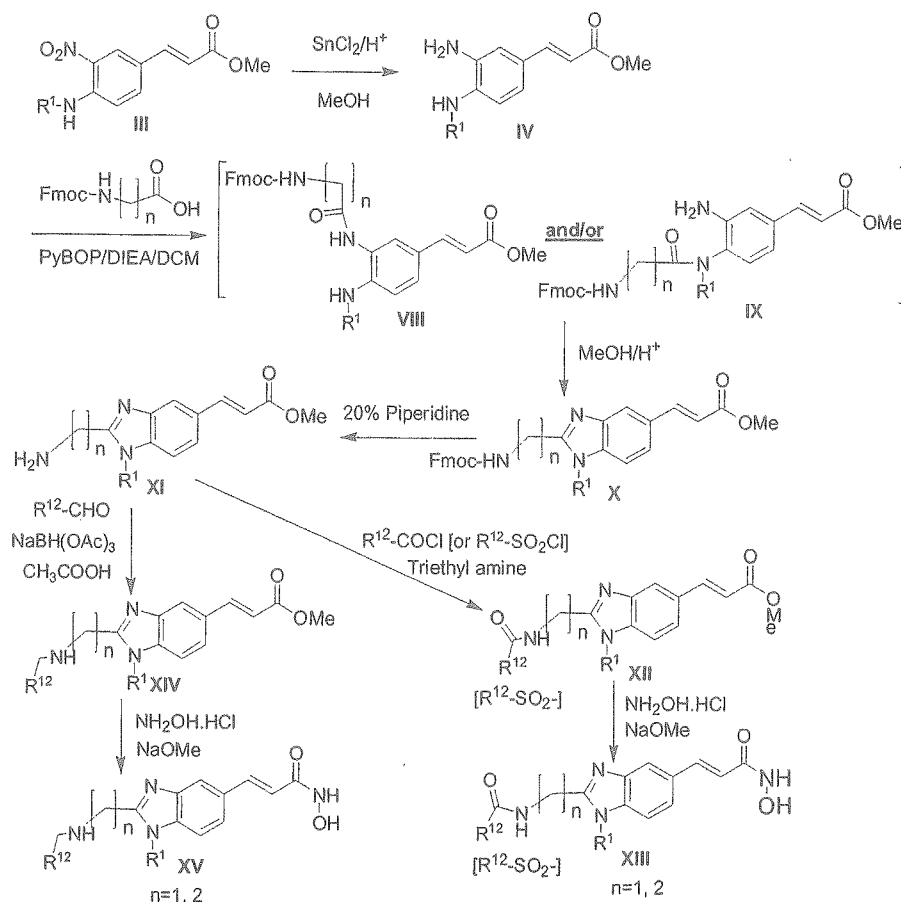
Scheme III
