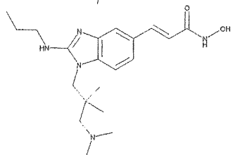
3-[1-(3-Dimethylamino-2,2-dimethyl-propyl)-2- propylamino-1H-benzimidazol-5-yl]-N-hydroxy- acrylamide
