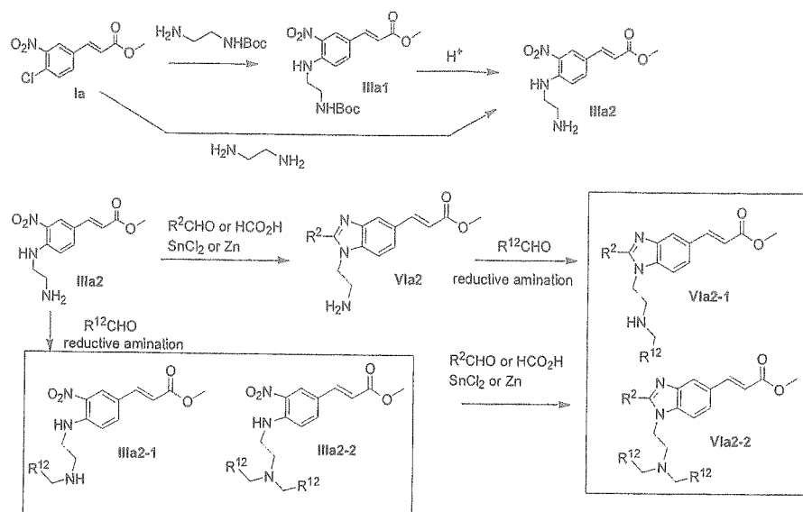
Scheme V
