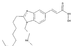
N-Hydroxy-3-[1-(2-methylamino-ethyl)-2-octyl-1H-benzimidazol-5-yl]-acrylamide
