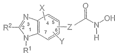
Formula (Ib)
