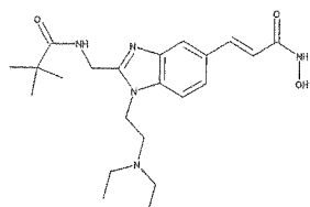
3-{1-(2-Diethylamino-ethyl)-2-[(2,2-dimethylpropionylamino)-methyl]-1H-benzoimidazol-5-yl}-N-hydroxy-acrylamide
