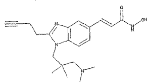
3-[2-But-3-ynyl-1-(3-dimethylamino-2,2-dimethyl-propyl)-1H-benzoimidazol-5-yl]-N-hydroxy-acrylamide
