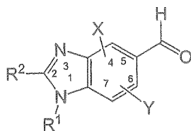
(B1)
