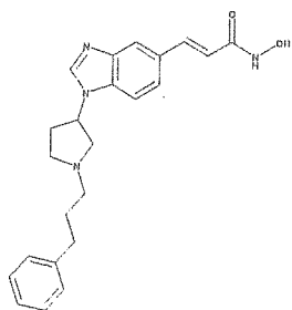
(E)-N-hydroxy-3-(1-(1-(3-phenylpropyl)pyrrolidin-3-yl)-1H-benzo[d]imidazol-5-yl)acrylamide
