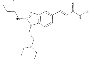
3-[1-(2-Diethylamino-ethyl)-2-propylamino-1H-benzimidazol-5-yl]-N-hydroxy-acrylamide
