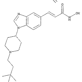
(E)-3-(1-(1-(3,3-dimethylbutyl)piperidin-4-yl)-1H-benzo[d]imidazol-5-yl)-N-hydroxyacrylamide
