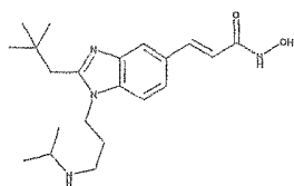
3-[2-(2,2-Dimethyl-propyl)-1-(3-isopropylamino-propyl)-1H-benzoimidazol-5-yl]-N-hydroxy-acrylamide
