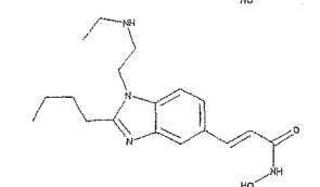
3-[2-Butyl-1-(2-ethylamino-ethyl)-1H-benzimidazol-5-yl]-N-hydroxy-acrylamide
