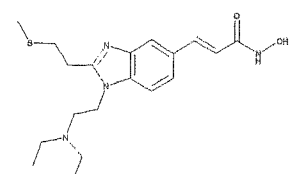
3-[1-(2-Diethylamino-ethyl)-2-(2-methylsulfanyl-ethyl)-1H-benzimidazol-5-yl]-N-hydroxy-acrylamide
