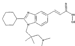
3-[2-Cyclohexyl-1-(3-dimethylamino-2,2-dimethyl-propyl)-1H-benzoimidazol-5-yl]-N-hydroxy-acrylamide
