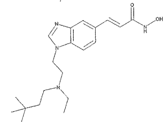
3-(1-(2-((3,3-Dimethyl-butyl)-ethyl-amino)-ethyl)-1H-benzoimidazol-5-yl)-N-hydroxy-acrylamide
