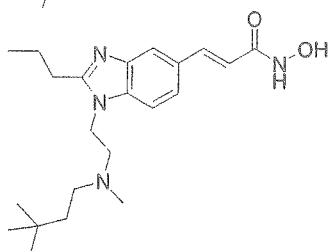
3-(1-{2-[(3,3-Dimethyl-butyl)-methyl-amino]-ethyl}-2-propyl-1H-benzoimidazol-5-yl)-N-hydroxy-acrylamide
