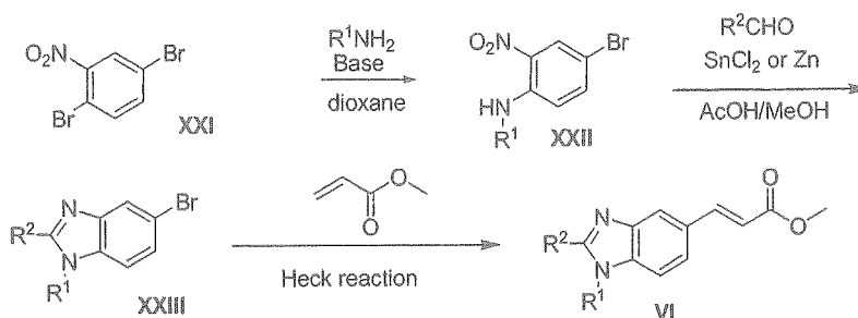
Scheme VII
