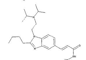
3-[2-Butyl-1-(2-diisopropylamino-ethyl)-1H-benzimidazol-5-yl]-N-hydroxy-acrylamide
