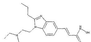
3-[1-(2-Diethylamino-ethyl)-2-propyl-1H-benzimidazol-5-yl]-N-hydroxy-acrylamide
