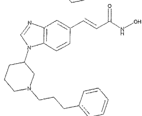
(E)-N-hydroxy-3-(1-(1-(3-phenylpropyl)piperidin- 3-yl)-1H-benzo[d]imidazol-5-yl)acrylamide
