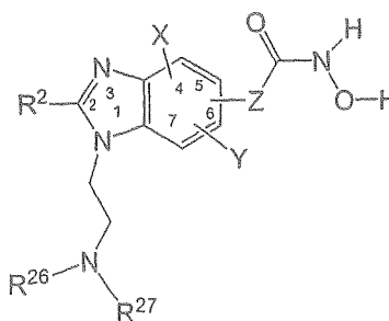
Formula (IIc)
