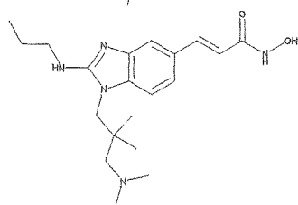
3-[1-(3-Dimethylamino-2,2-dimethyl-propyl)-2-propylamino-1H-benzoimidazol-5-yl]-N-hydroxy-acrylamide
