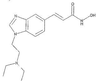
(E)-3-(1-(2-(diethylamino)ethyl)-1H-benzo[d]imidazol-5-yl)-N-hydroxyacrylamide
