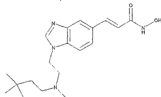
3-(1-{2-[(3,3-Dimethyl-butyl)-methyl-amino]-ethyl}-1H-benzoimidazol-5-yl)-N-hydroxy-acrylamide
