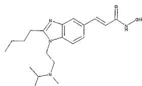
3-{2-Butyl-1-[2-(isopropyl-methyl-amino)-ethyl]-1H-benzimidazol-5-yl}-N-hydroxy-acrylamide
