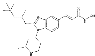
N-Hydroxy-3-[1-(3-isopropylamino-propyl)-2-(2,4,4-trimethyl-pentyl)-1H-benzimidazol-5-yl]-acrylamide
