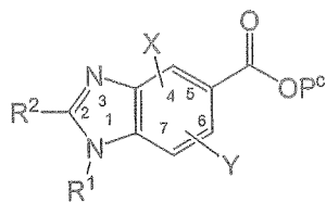
(B5)
