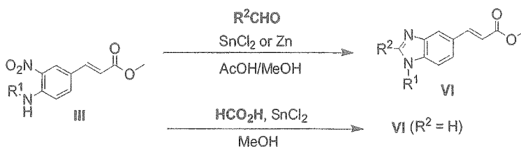
Scheme II
