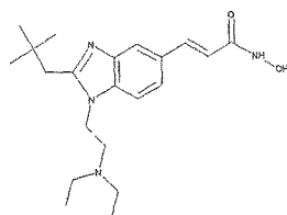
3-[1-(2-Diethylamino-ethyl)-2-(2,2-dimethyl-propyl)-1H-benzoimidazol-5-yl]-N-hydroxy-acrylamide
