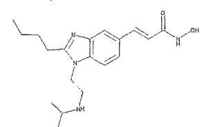
3-[2-Butyl-1-(2-isopropylamino-ethyl)-1H-benzimidazol-5-yl]-N-hydroxy-acrylamide
