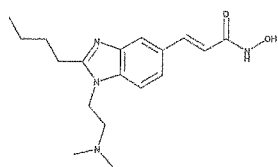
3-[2-Butyl-1-(2-dimethylamino-ethyl)-1H-benzoimidazol-5-yl]-N-hydroxy-acrylamide
