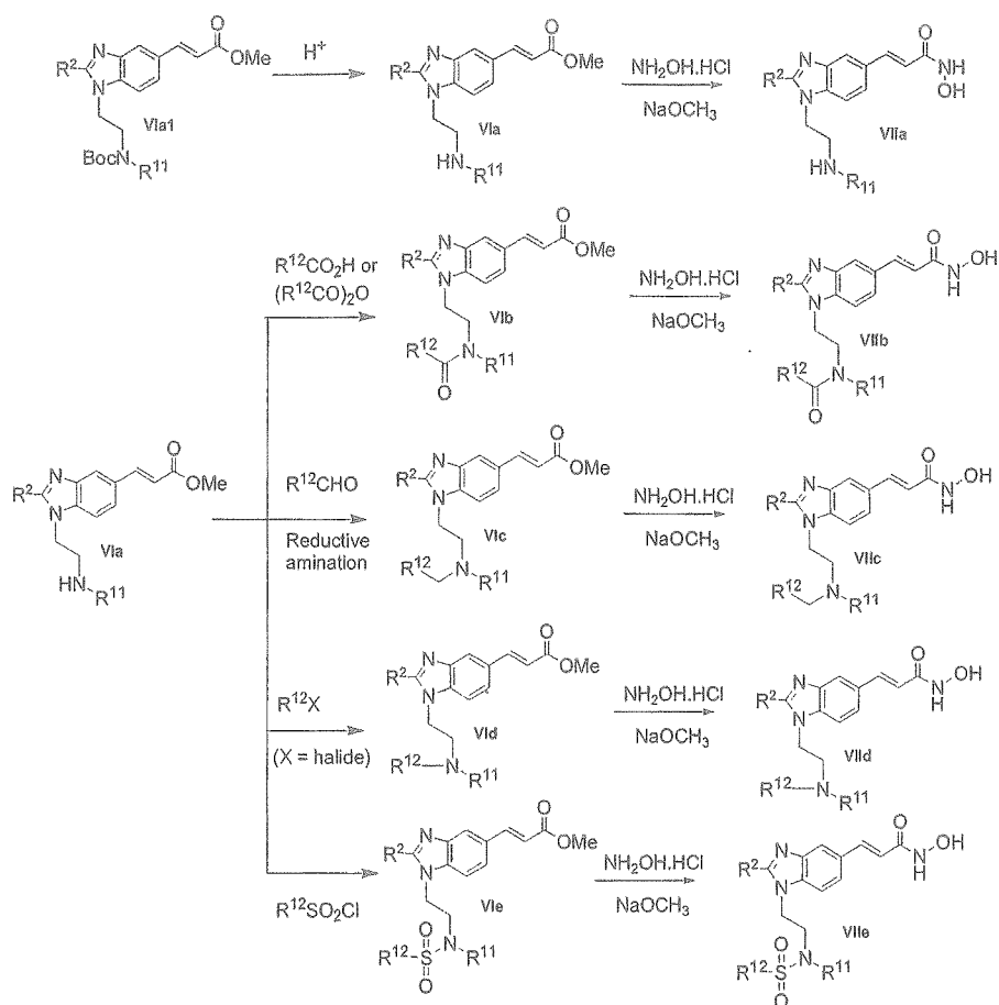
Scheme IV
