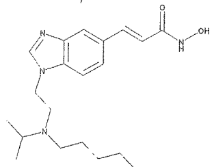
N-Hydroxy-3-{1-[2-(isopropyl-pentyl-amino)-ethyl]-1H-benzimidazol-5-yl}-acrylamide
