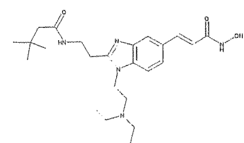
N-{2-[1-(2-Diethylamino-ethyl)-5-(2-hydroxycarbamoyl-vinyl)-1H-benzimidazol-2-yl]-ethyl}-3,3-dimethyl-butamide
