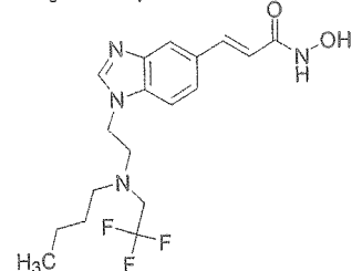
3-(1-{2-[Butyl-(2,2,2-trifluoro-ethyl)-amino]-ethyl}-1H-benzoimidazol-5-yl)-N-hydroxy-acrylamide
