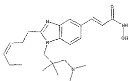
3-[1-(3-Dimethylamino-2,2-dimethyl-propyl)-2-hex-3-enyl-1H-benzoimidazol-5-yl]-N-hydroxy-acrylamide
