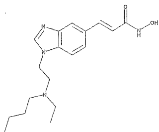
3-{1-[2-(Butyl-ethyl-amino)-ethyl]-1H-benzoimidazol-5-yl}-N-hydroxy-acrylamide
