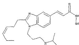
3-[2-Hex-3-enyl-1-(3-isopropylamino-propyl)-1H-benzimidazol-5-yl]-N-hydroxy-acrylamide
