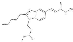
3-{1-[2-(Ethyl-methyl-amino)-ethyl]-2-pentyl-1H-benzoimidazol-5-yl}-N-hydroxy-acrylamide
