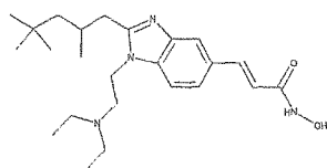
3-[1-(2-Diethylamino-ethyl)-2-(2,4,4-trimethyl-pentyl)-1H-benzimidazol-5-yl]-N-hydroxy-acrylamide
