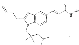
3-[2-But-3-enyl-1-(3-dimethylamino-2,2-dimethyl-propyl)-1H-benzoimidazol-5-yl]-N-hydroxy-acrylamide
