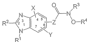
Formula (Ic)
