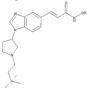
3-{1-[1-(3,3-Dimethyl-butyl)-pyrrolidin-3-yl]-1H-benzoimidazol-5-yl}-N-hydroxy-acrylamide
