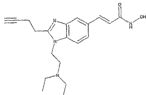
3-[2-But-3-ynyl-1-(2-diethylamino-ethyl)-1H-benzoimidazol-5-yl]-N-hydroxy-acrylamide
