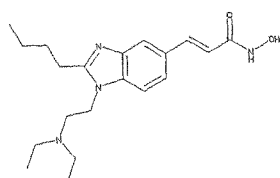
3-[2-Butyl-1-(2-diethylamino-ethyl)-1H-benzoimidazol-5-yl]-N-hydroxy-acrylamide
