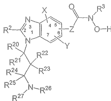
Formula (IIIa)
