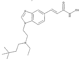
3-(1-{2-[(3,3-Dimethyl-butyl)-ethyl-amino]-ethyl}- 1H-benzimidazol-5-yl)-N-hydroxy-acrylamide
