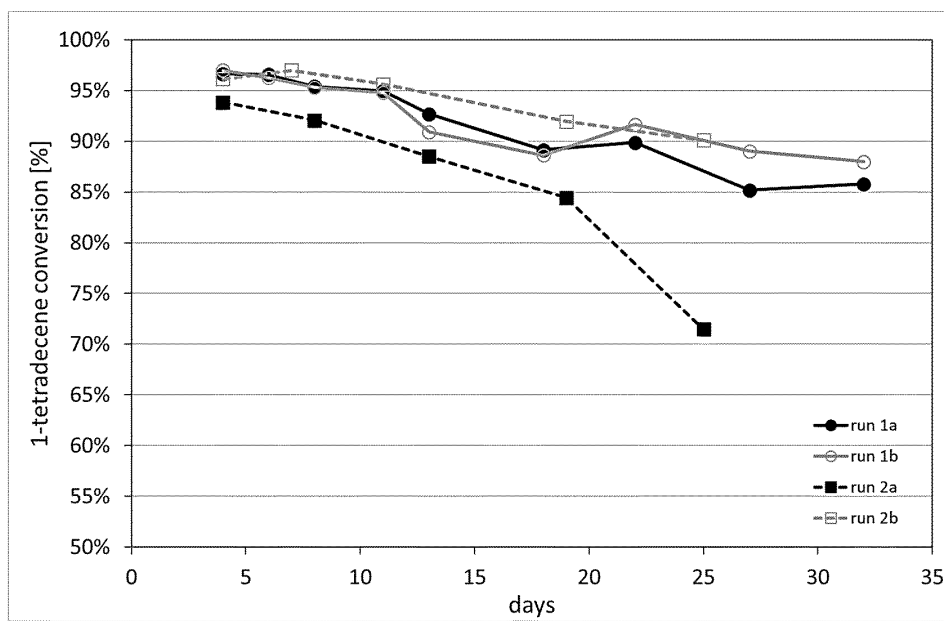
Figure 1: Comparison of long-term stability tests ( ^{13}\text{C} -NMR) of the 1-tetradecene conversion in all reactors and experiments
