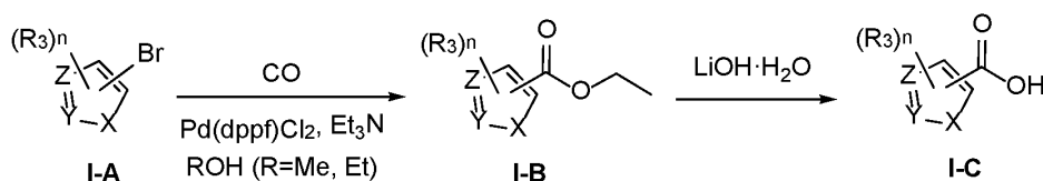
SCHEME I-1
