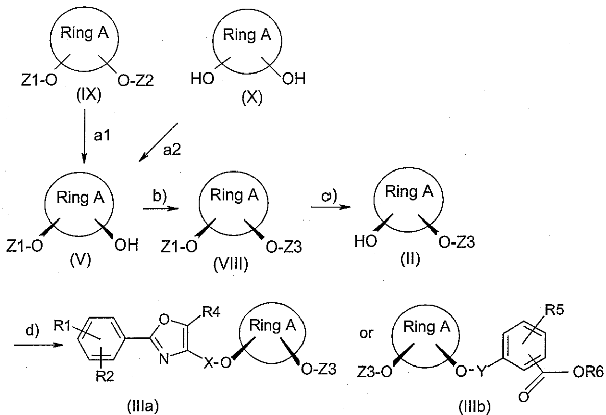
Scheme I
