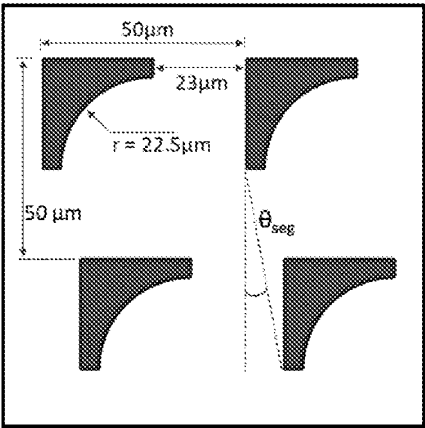
(b) DLD Device 2: L -1 Shape
