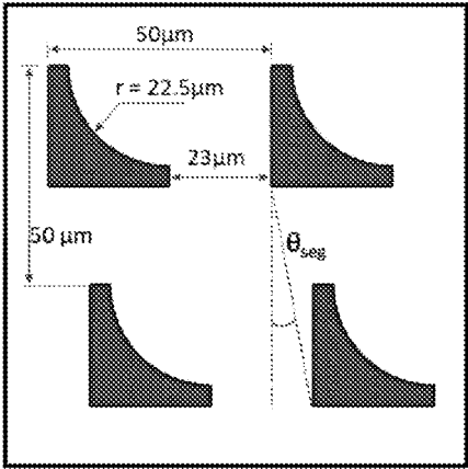
(a) DLD Device 1: L Shape
