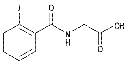
o -iodohippuran
