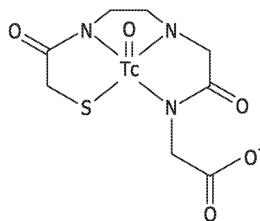
^{99m}\text{Tc} -MAG3
