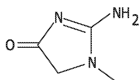
creatinine
