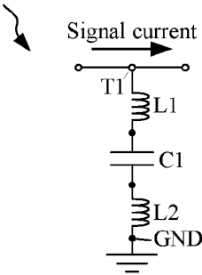
302 2-Terminal Circuit
