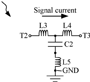
304 3-Terminal Circuit
