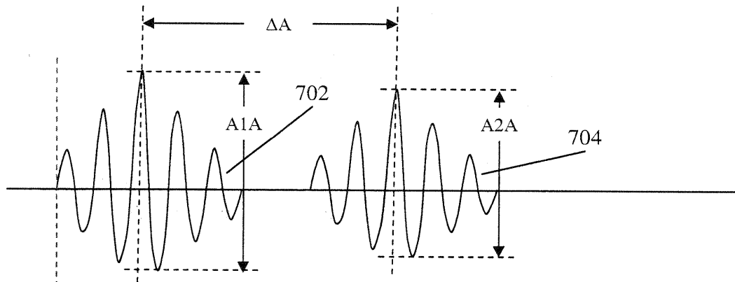
Figure 7a. Waveform captured at antenna A
