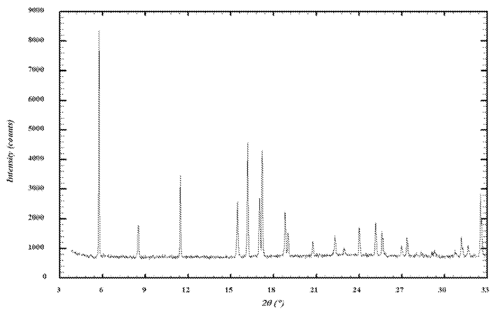
FIG. 4. XRPD pattern of form 4
