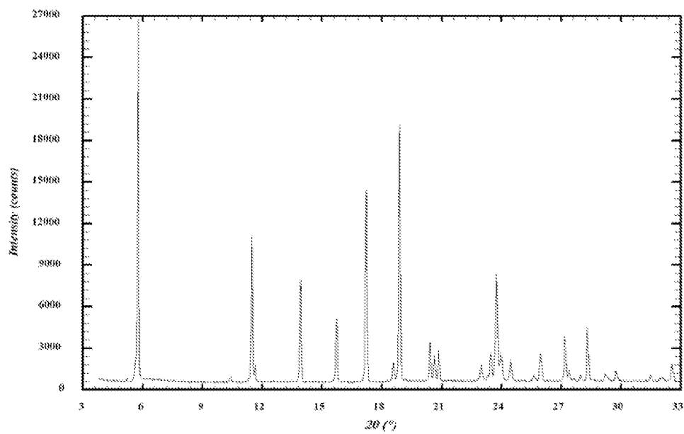
FIG. 1. XRPD pattern of form 1
