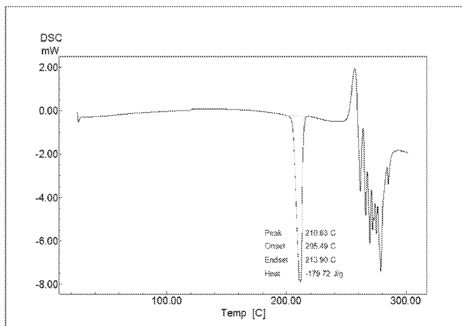
FIG. 6. DSC of form 1
