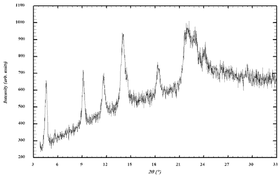
FIG. 5. XRPD pattern of amorphous form
