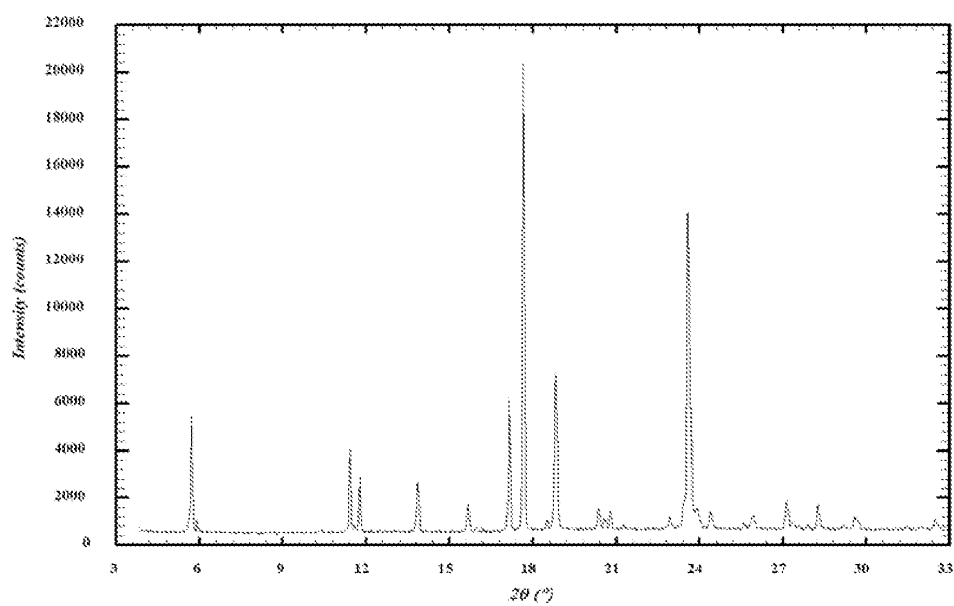
FIG. 3. XRPD pattern of form 1 + form 3
