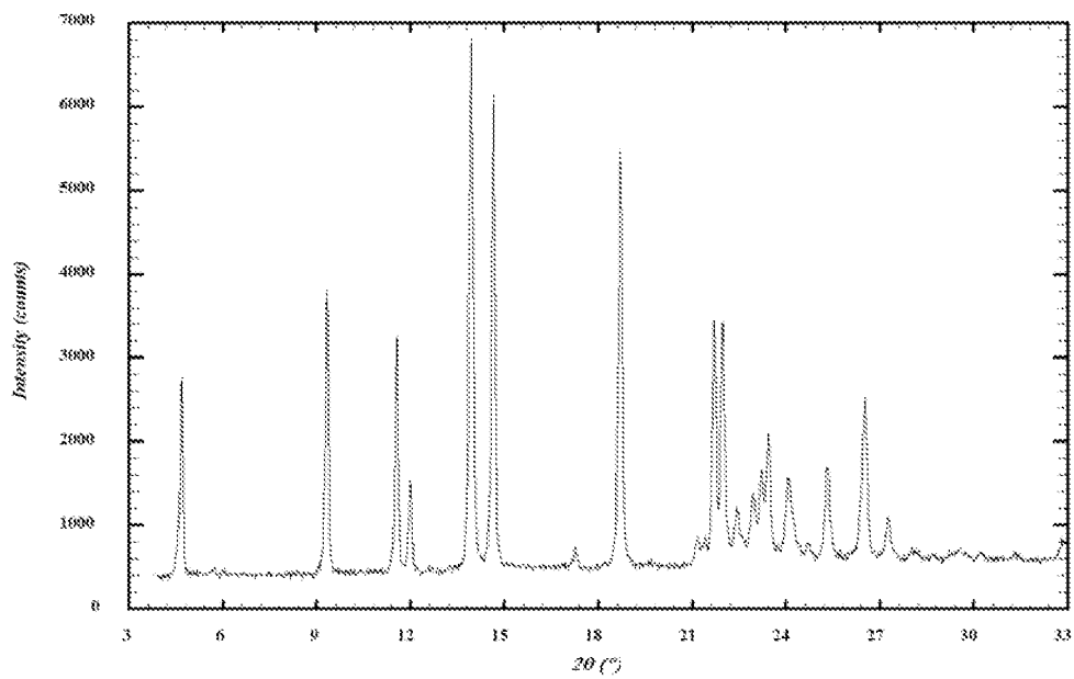
FIG. 2. XRPD pattern of form 2
