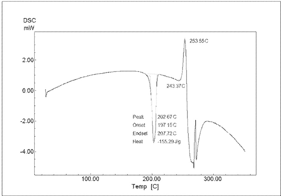
FIG. 7. DSC of form 2
