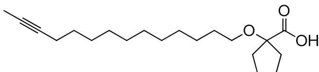
2-ethyl-2-(tetradec-12-yn-1-yloxy)butanoic acid ( 53 )
