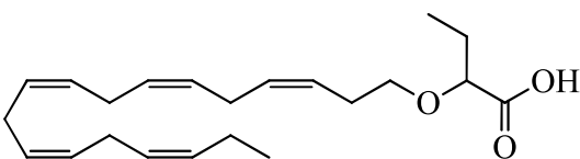
2-((3Z,6Z,9Z,12Z,15Z)-octadeca-3,6,9,12,15-pentaenyloxy)butanoic acid, or
