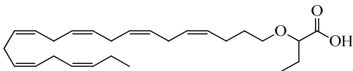
2-((4Z,7Z,10Z,13Z,16Z,19Z)-docosa-4,7,10,13,16,19-hexaen-1-yloxy)butanoic acid ( 19 )
