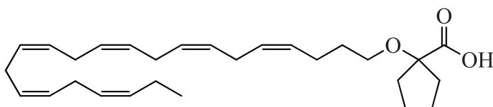
2-((4Z,7Z,10Z,13Z,16Z,19Z)-docosa-4,7,10,13,16,19-hexaen-1-yloxy)-2-ethylbutanoic acid ( 20 )
