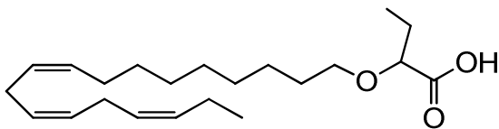
2-((9Z,12Z,15Z)-octadeca-9,12,15-trienyloxy)butanoic acid;
