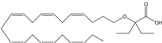
2-ethyl-2-((4Z,7Z,10Z,13Z,16Z,19Z)-docosa-4,7,10,13,16,19-hexaenyloxy)butanoic acid,
