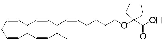
2-ethyl-2-((5Z,8Z,11Z,14Z,17Z)-icosa-5,8,11,14,17-pentaenyloxy)butanoic acid,
