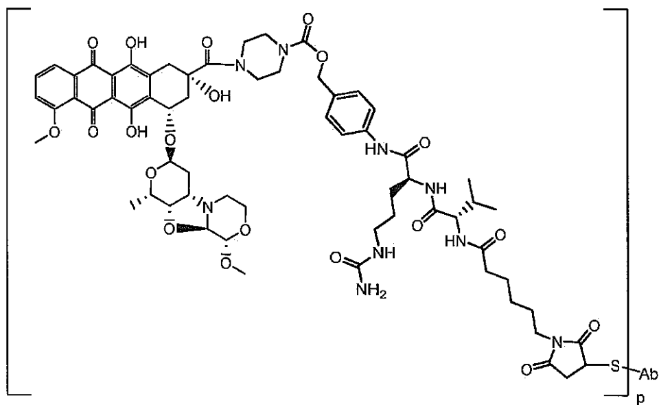
PNU-159682-val-cit-PAB-Ab;
