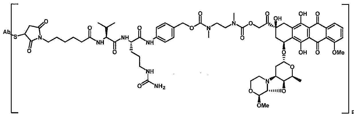
PNU-159682-val-cit-PAB-spacer-Ab;
