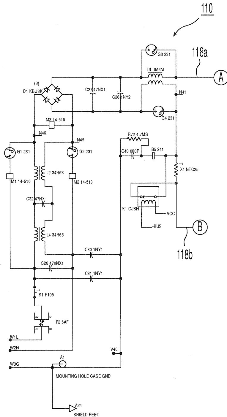
EMI Filter &amp; Rectifier Bridge
