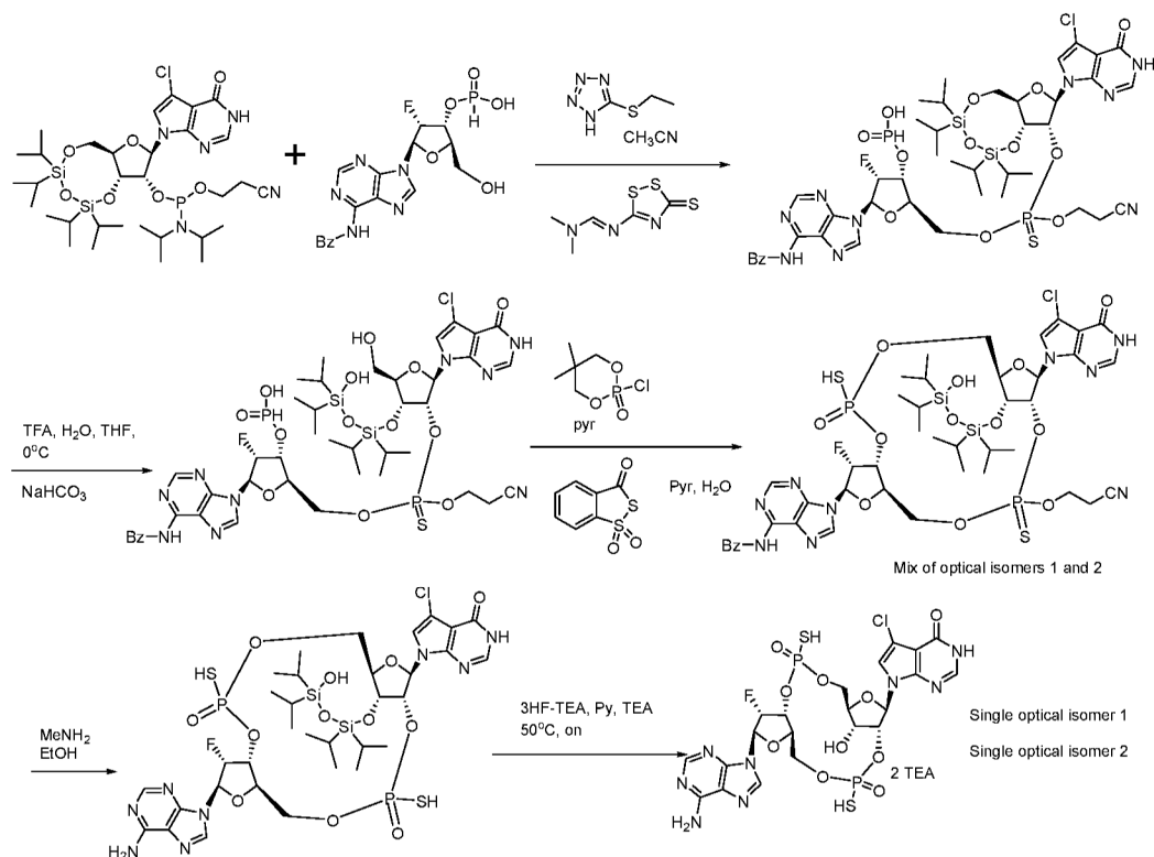
A) (6aR,8R,9R,9aR)-8-(5-chloro-4-oxo-3,4-dihydro-7H-pyrrolo[2,3-d]pyrimidin-7-yl)-2,2,4,4-tetraisopropyltetrahydro-6H-furo[3,2-f][1,3,5,2,4]trioxadisilocin-9-yl 2-cyanoethyl diisopropylphosphoramidoite
