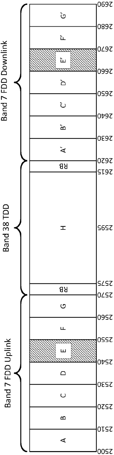
Fig. 16a (Prior Art)
