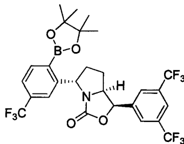
(1R,5S,7aS)-1-(3,5-bis(trifluoromethyl)phenyl)-5-(2-(4,4,5,5-tetramethyl-1,3,2-dioxaborolan-2-yl)-5-(trifluoromethyl)phenyl)tetrahydropyrrolo[1,2-c]oxazol-3(1H)-one
