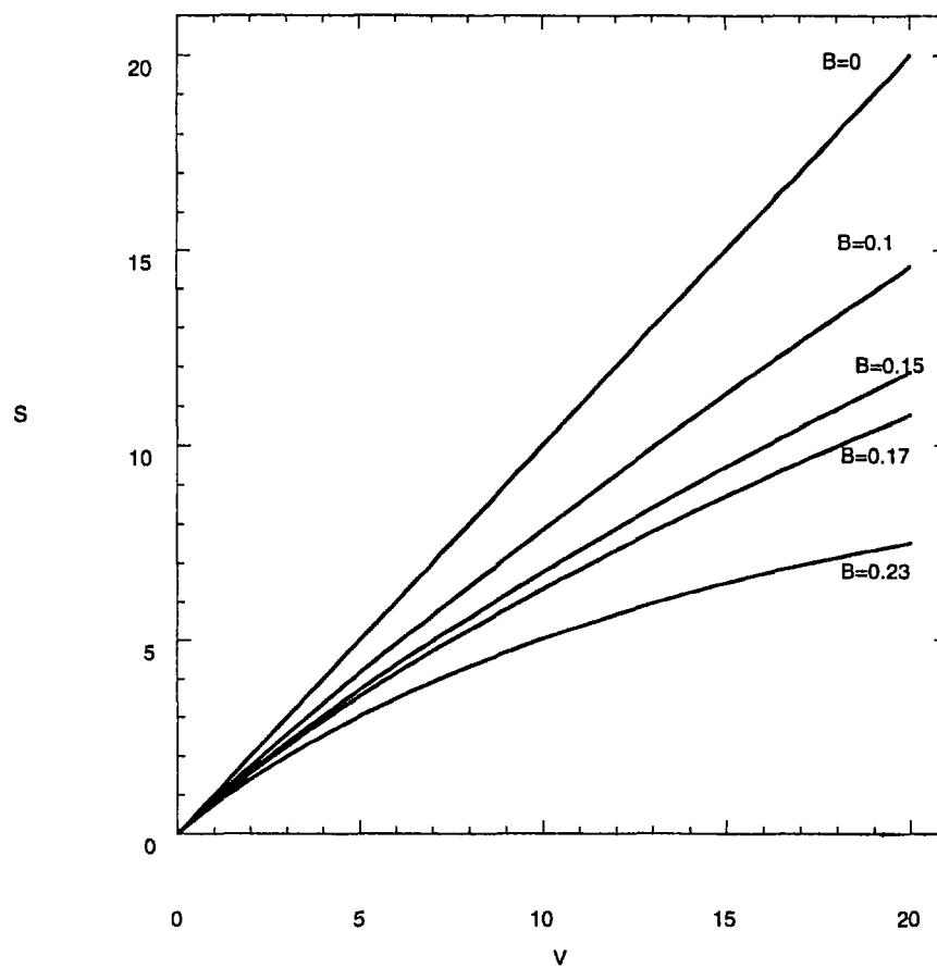
Scattering coefficient versus pigment volume concentration
