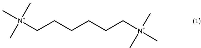
N,N,N',N',N',N'-Hexamethylhexamethylenediammonium or hexamethonium cation
