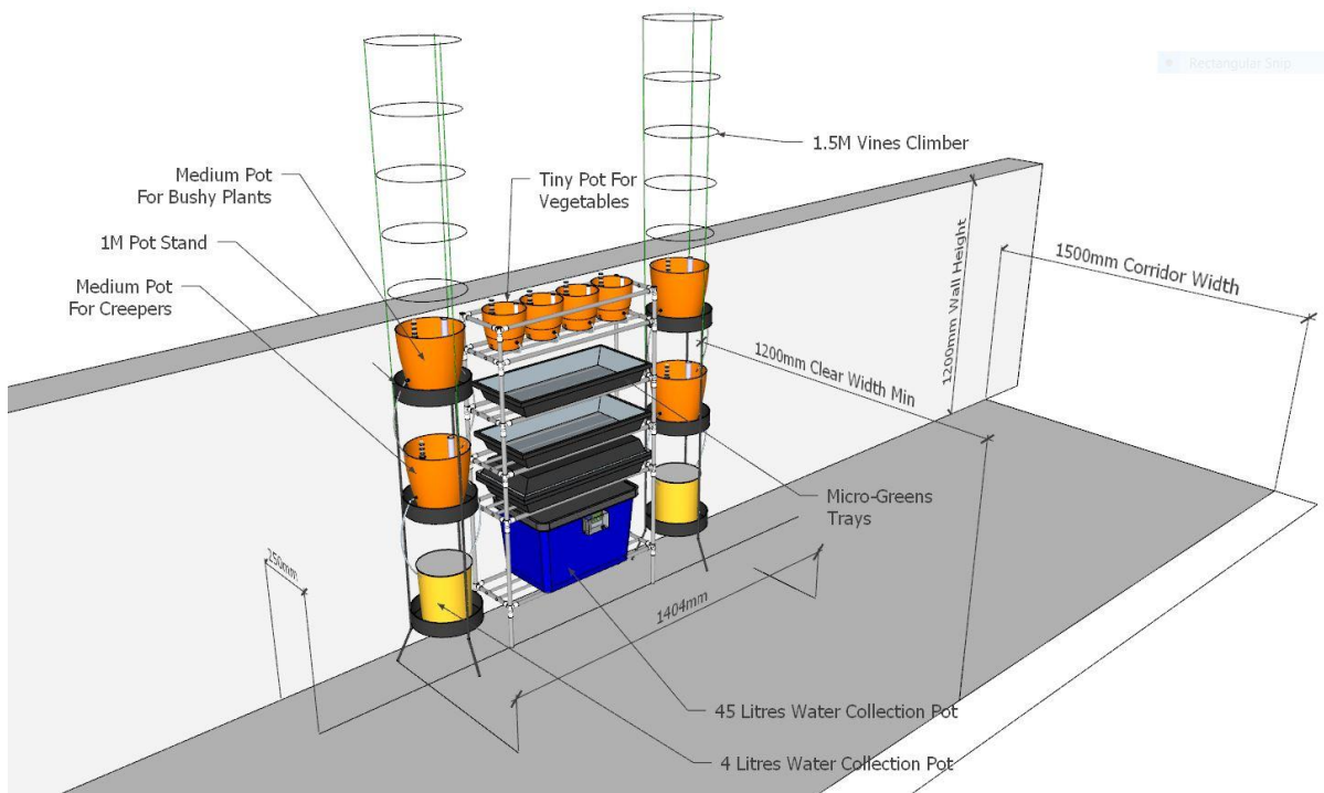
3D View of a basic module of the Grow System
