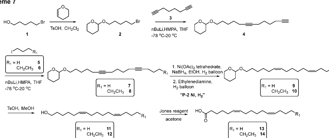
Scheme 7
