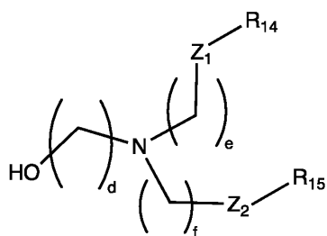
Formula VIII
