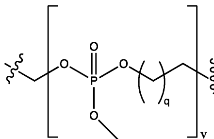
Formula I-A'
