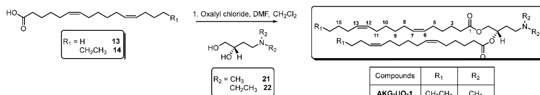
Scheme 9
