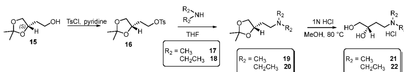
Scheme 8
