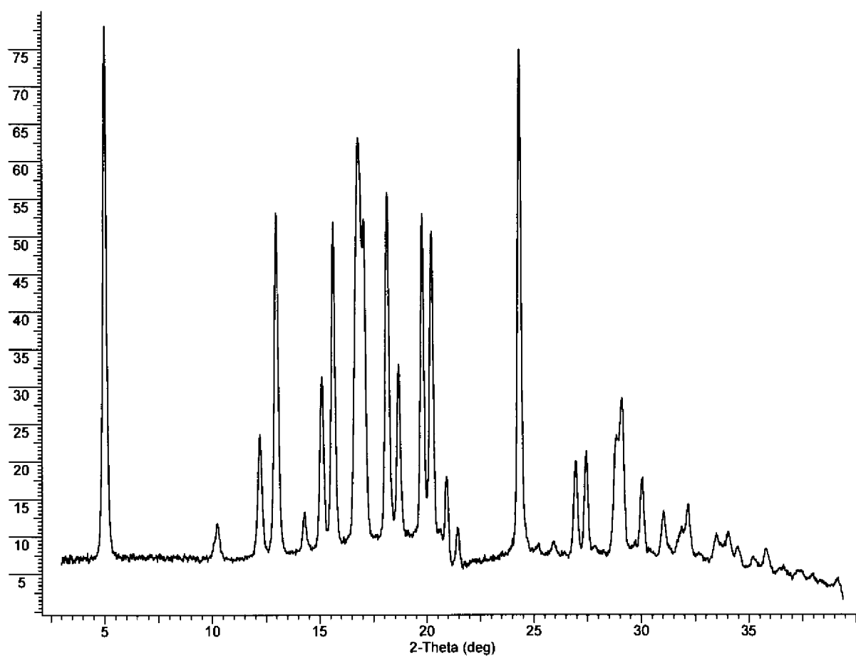
Figure 6: Malonate
