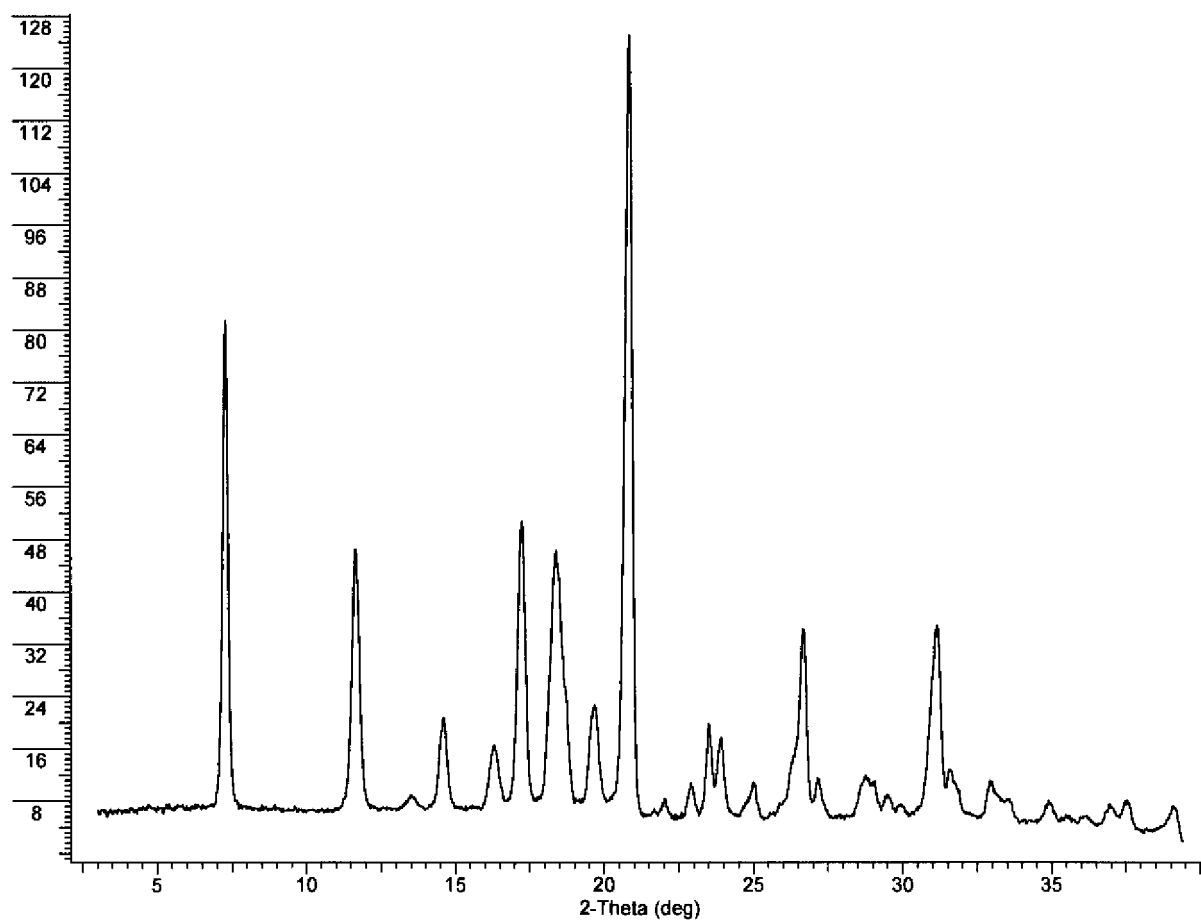
Figure 3: Hydrochloride
