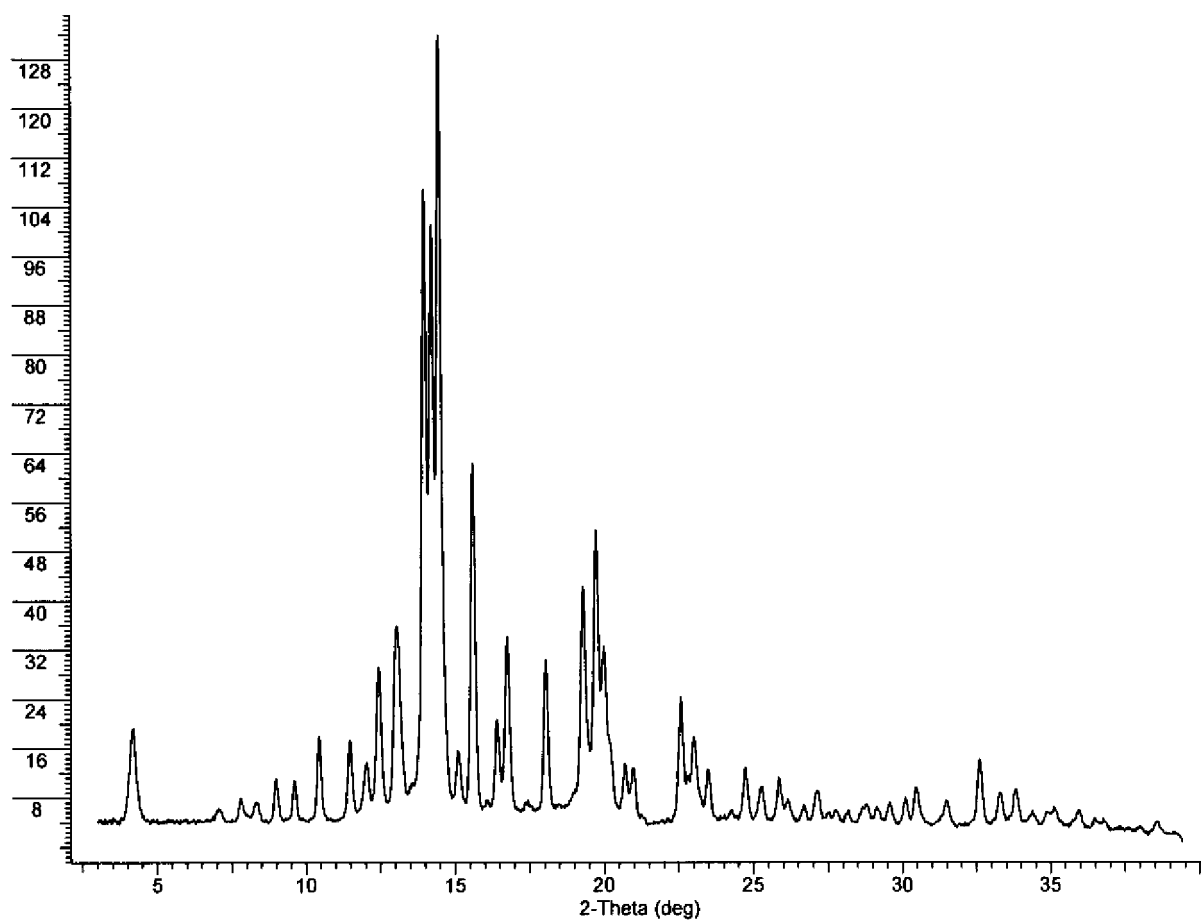
Figure 4B: Phosphate, Form B
