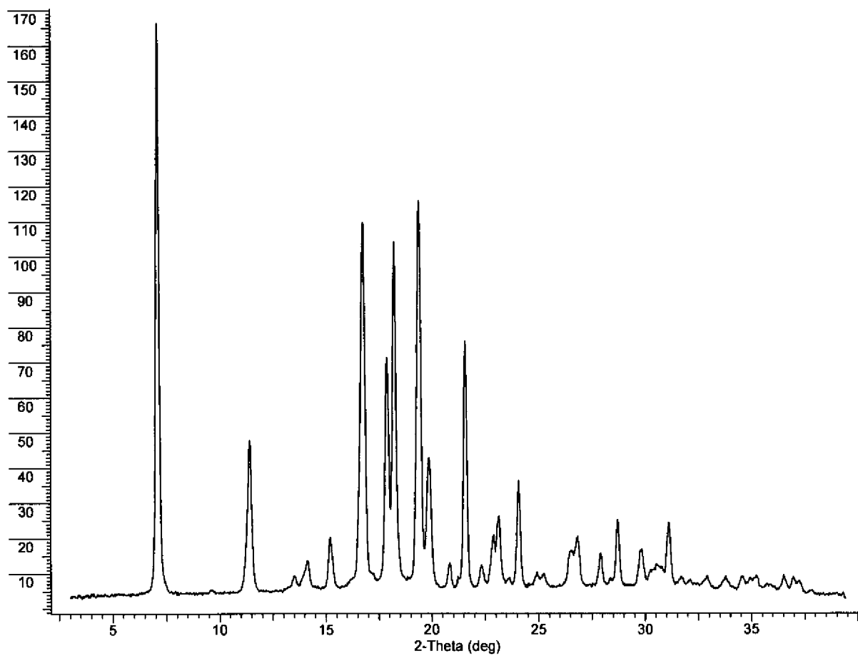
Figure 7B: Free base, Form B
