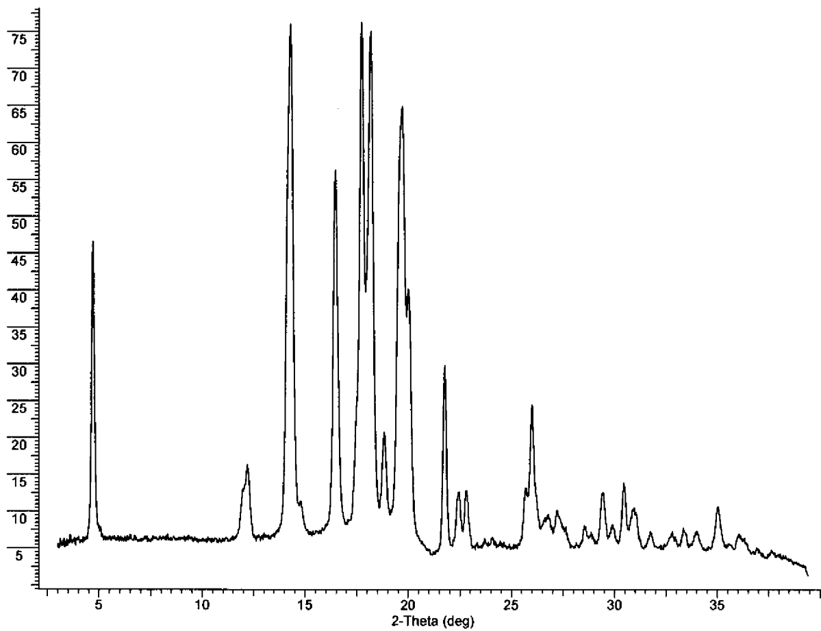
Figure 4A: Phosphate, Form A
