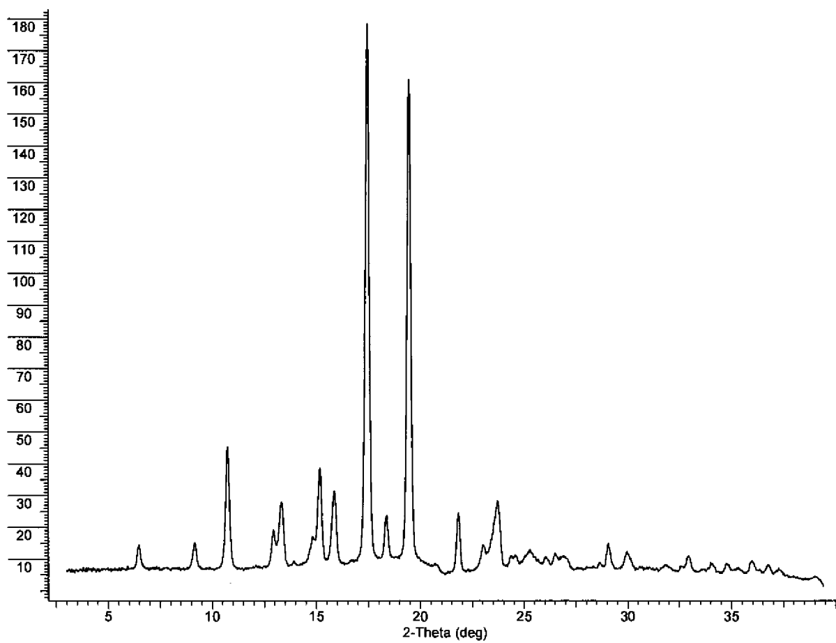
Figure 5A: Succinate, Form A
