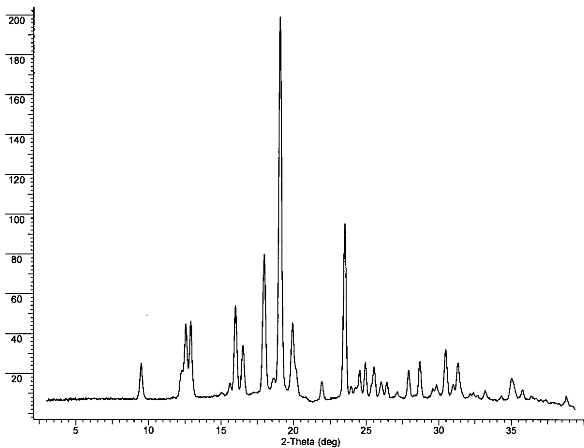
Figure 2: Maleate
