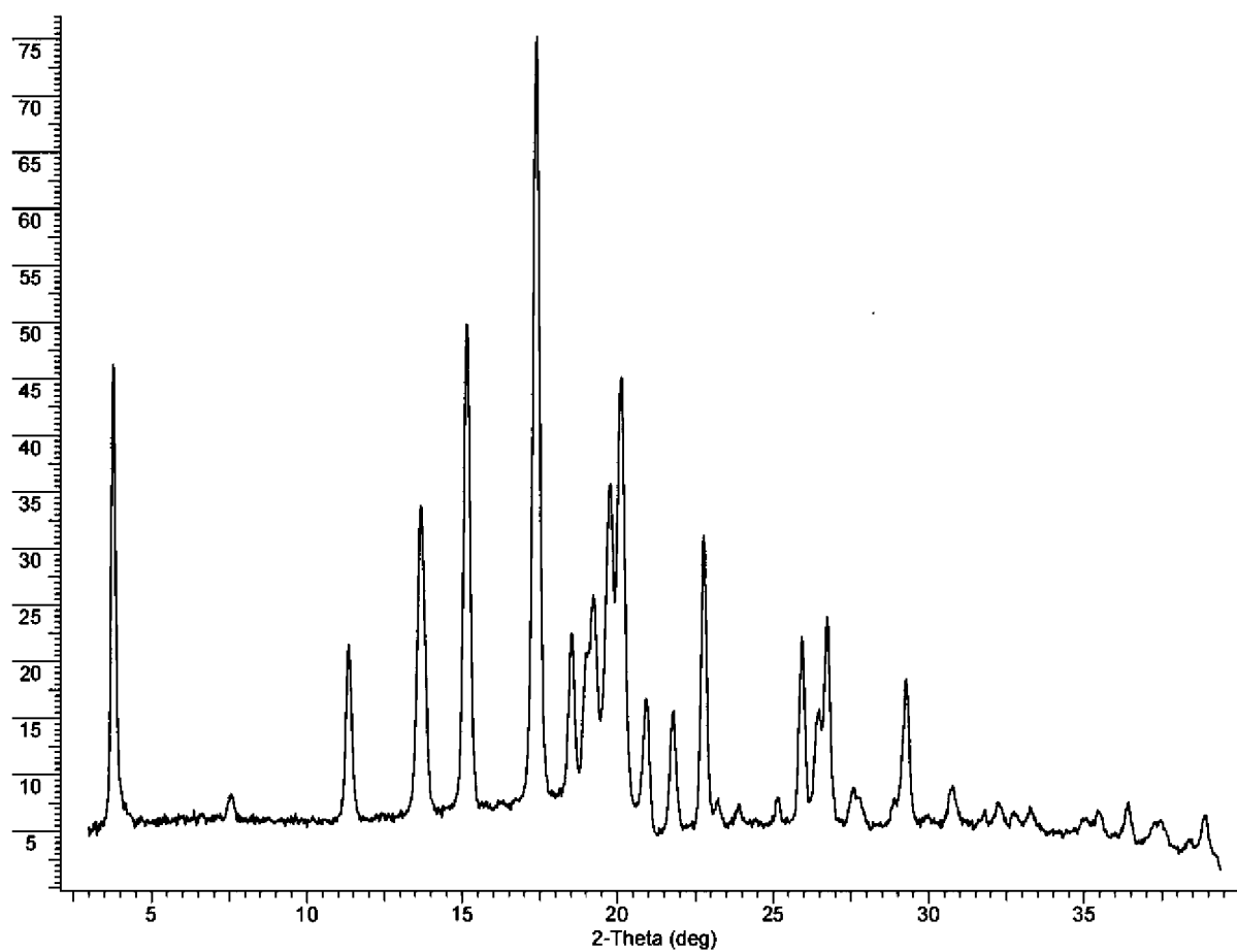
Figure 1: Fumarate
