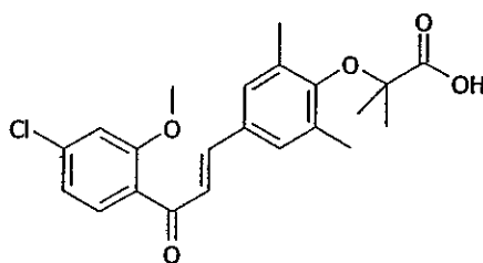
1-[2-methoxy-4-chlorophenyl]-3-[3,5-dimethyl-4-carboxydimethylmethoxyphenyl]prop-2-en-1-one
