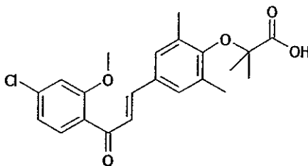
1-[2-methoxy-4-chlorophenyl]
