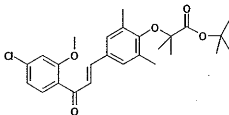
1-[2-methoxy-4-chlorophenyl]
