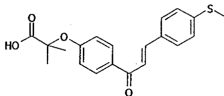
1-[4-carboxydimethylmethoxyphenyl]-3-[4-methylthiophenyl]prop-2-en-1-one
