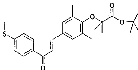
1-[4-methylthiophenyl]-3-[3,5-dimethyl-4-tert-butyloxycarbonyldimethylmethoxyphenyl]prop-2-en-1-one (Compound 8)
