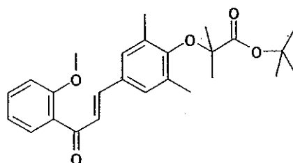
1-[2-methoxyphenyl]-3-[3,5-dimethyl-4-tert-butylloxycarbonyldimethylmethoxyphenyl]prop-2-en-1-one (Compound 5)
