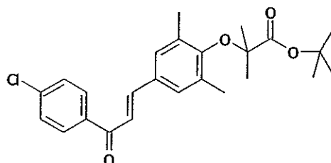
1-[4-chlorophenyl]-3-[3,5-dimethyl-4-tert-butylloxycarbonyldimethylmethoxyphenyl]prop-2-en-1-one (Compound 2)
