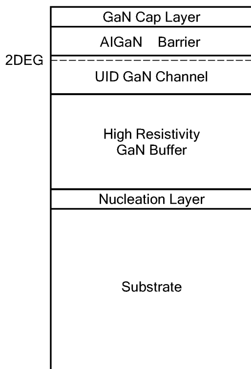
FIG. 1 PRIOR ART
