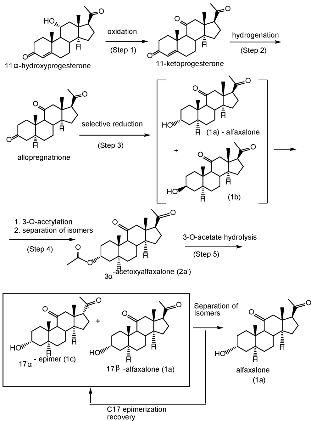
SCHEME 1. Preparation of Alfaxalone
