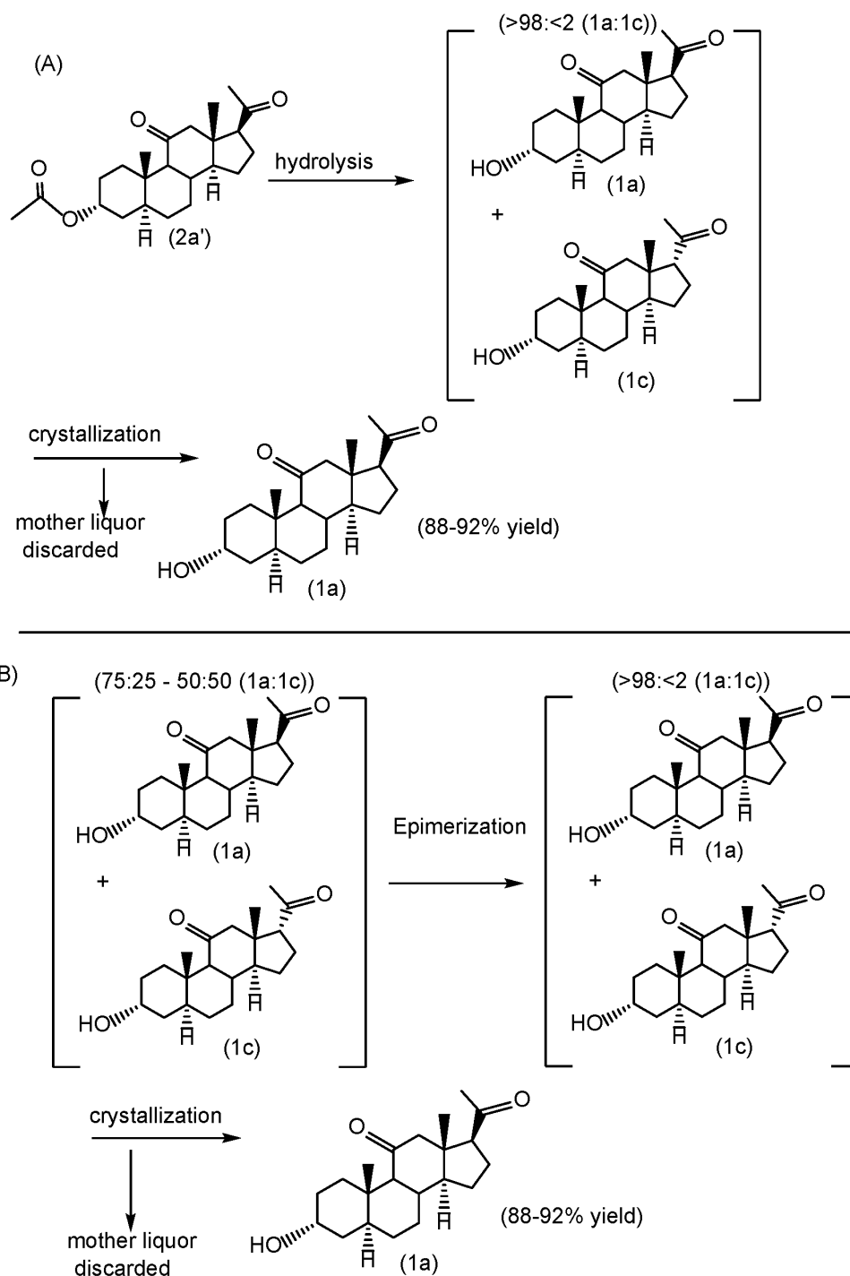
SCHEME 4. Hydrolysis of 3 \alpha -acetoxyalfaxalone (2a') and Hydrolysis of Crude 17 \alpha :17 \beta -enantiomers (1c:1a) to Prepare Alfaxalone (1a) - (Step 5 of Scheme 1)
