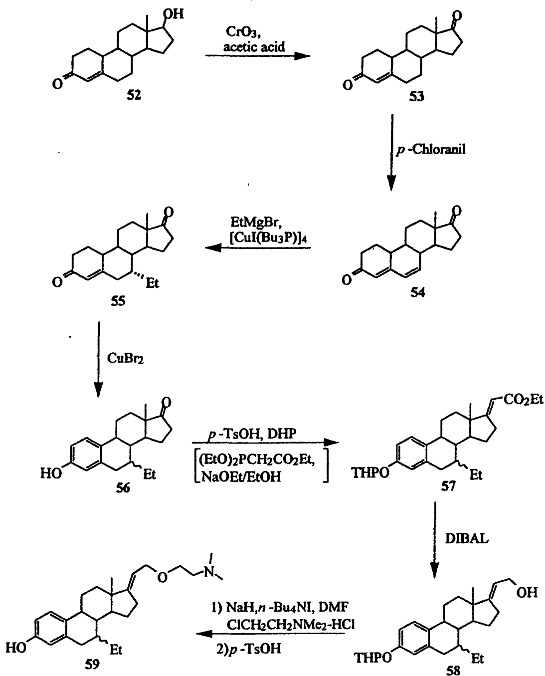
Scheme 11
