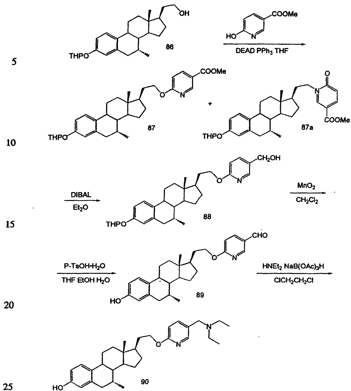
Scheme 19
