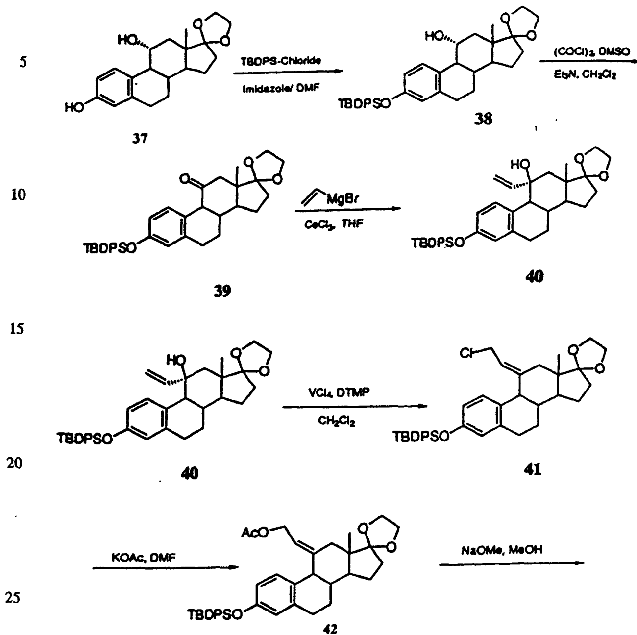
Scheme 8
