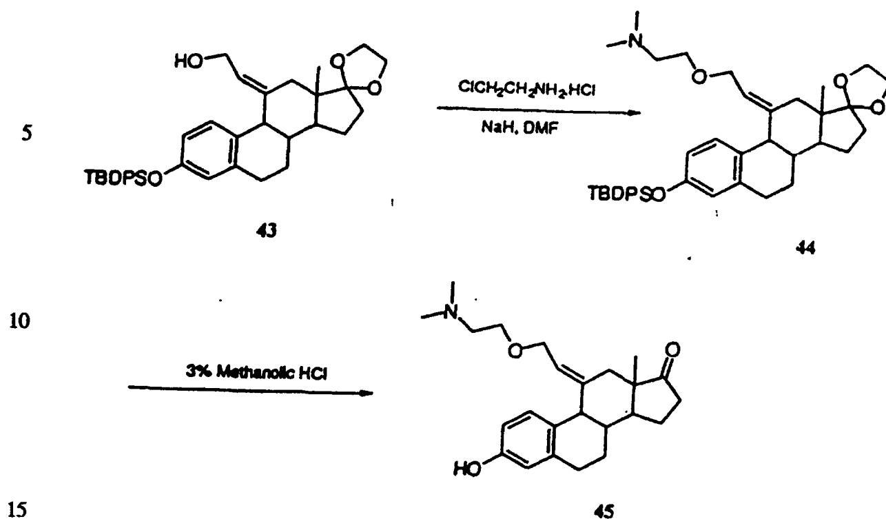
Scheme 8, continued
