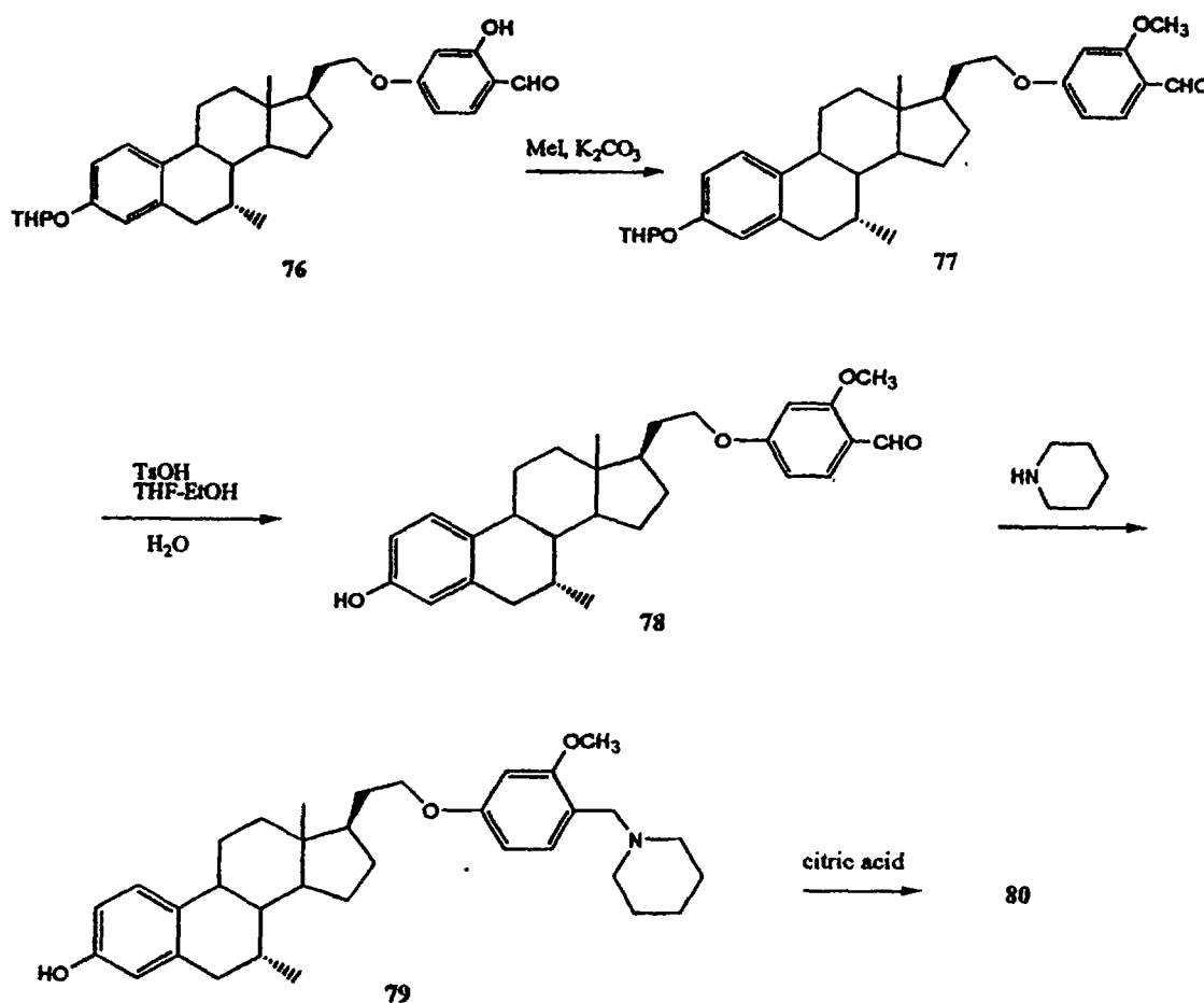
Scheme 16
