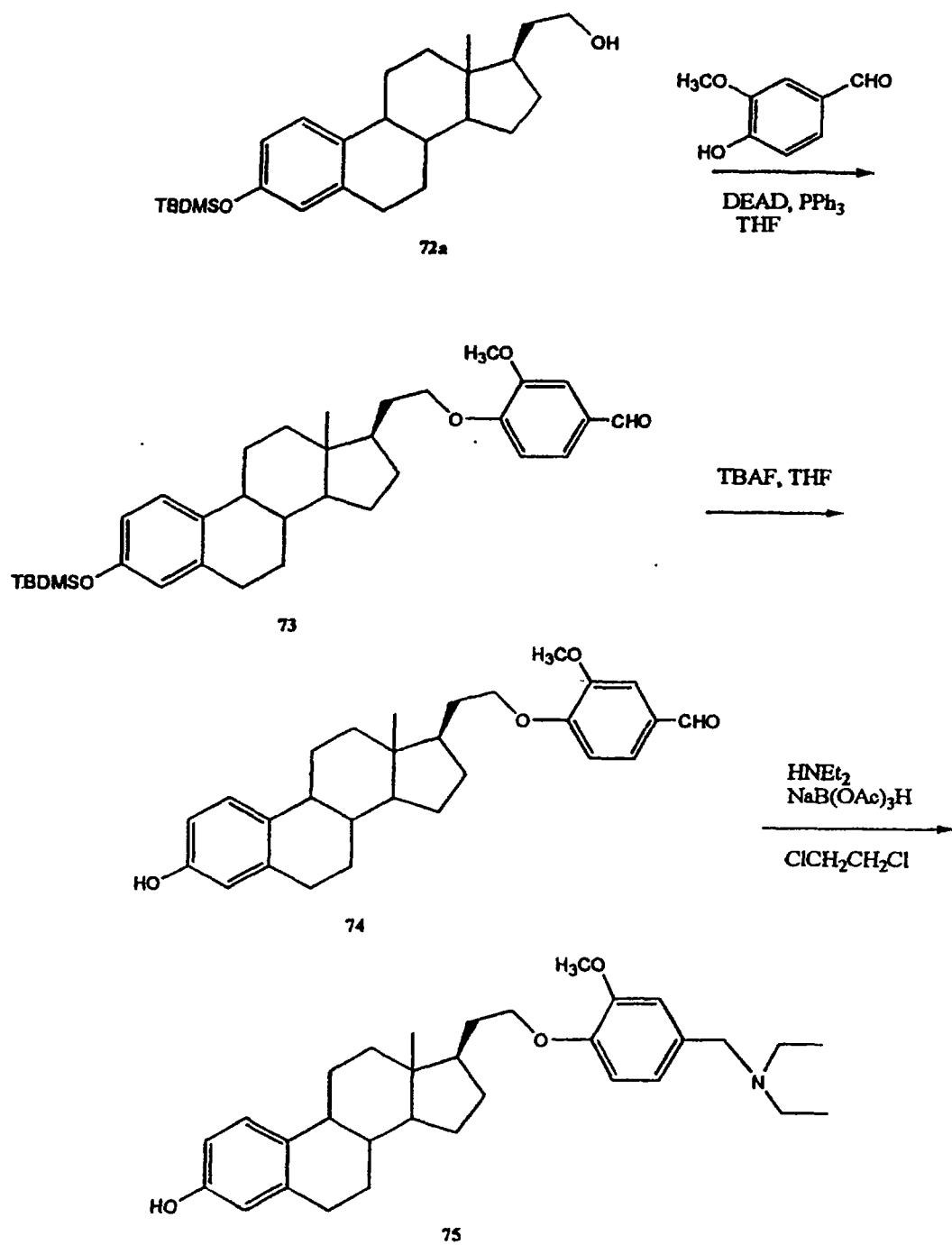
Scheme 15
