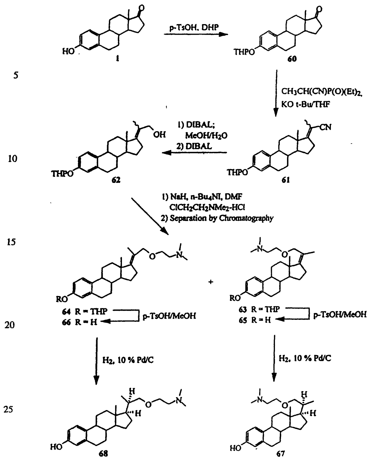
Scheme 12
