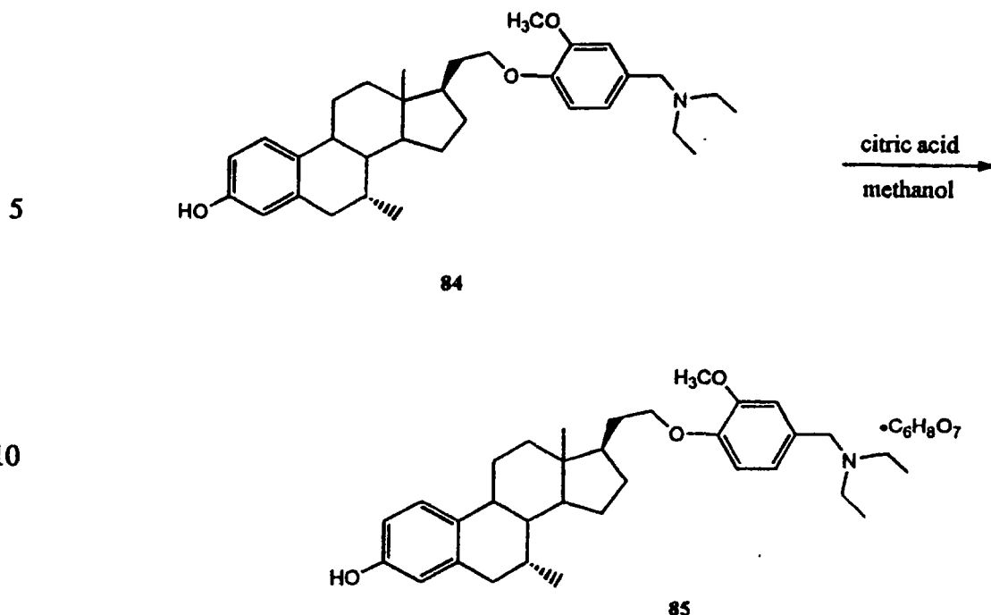
Scheme 18
