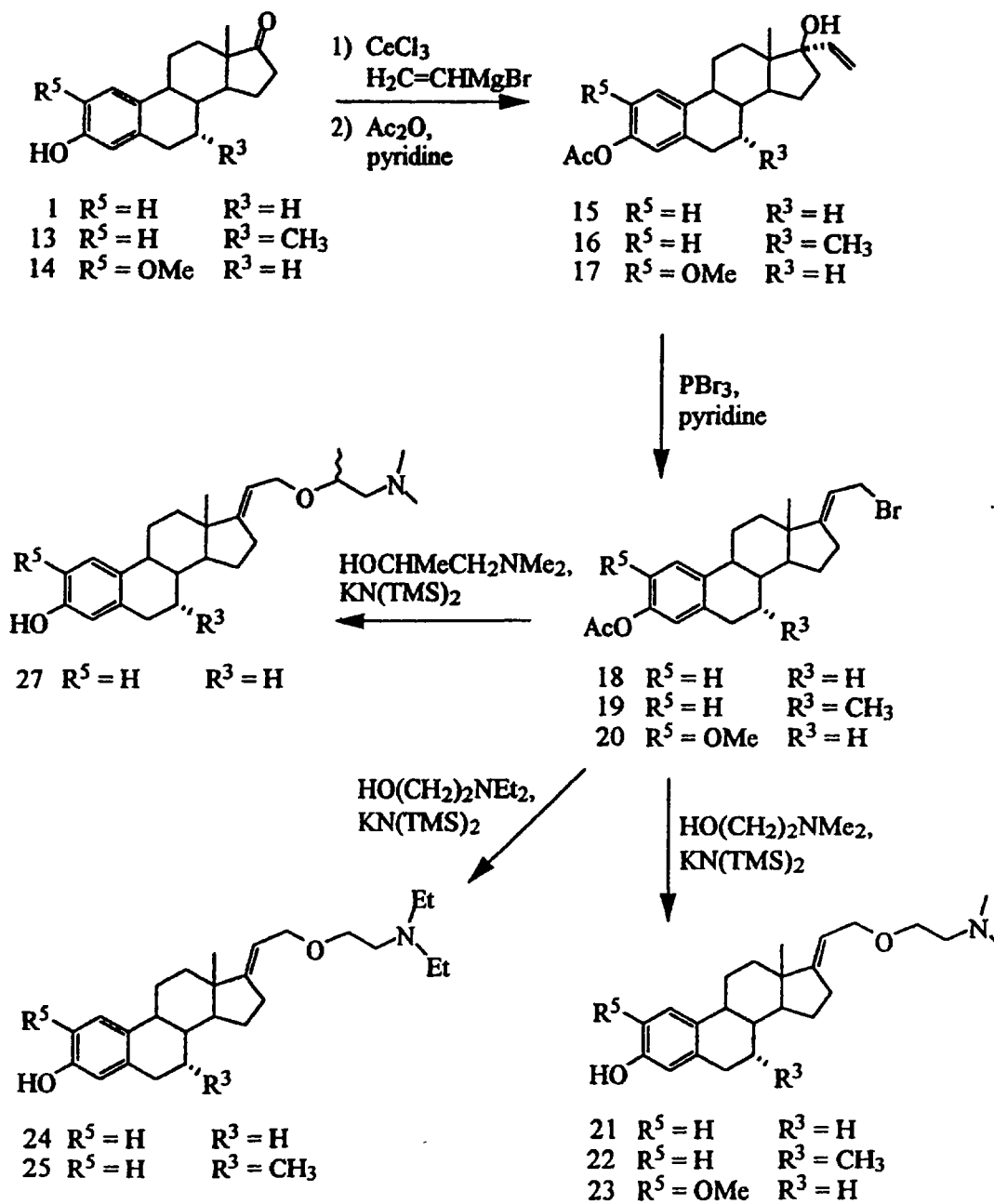
Scheme 4
