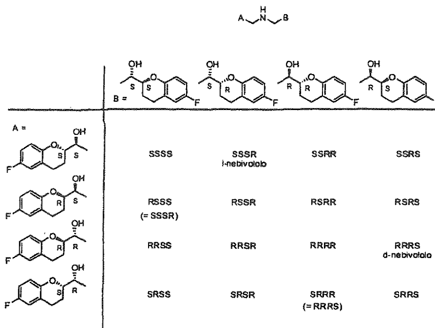
Scheme 2. Possible stereoisomers for Nebivolol
