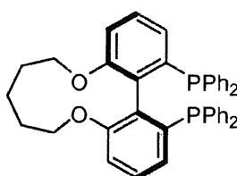
(S)-C5-TunePhos
