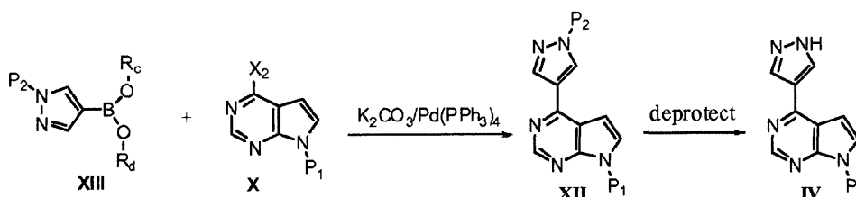
Scheme 11
