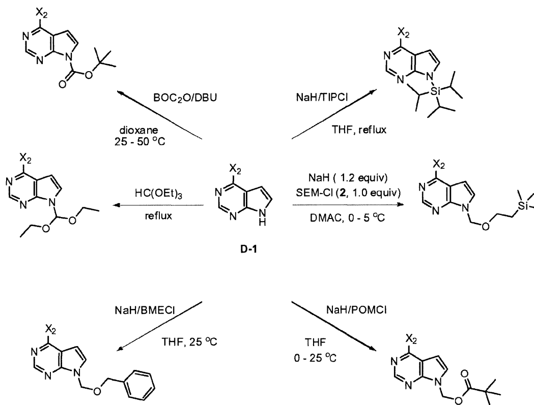
Scheme 13
