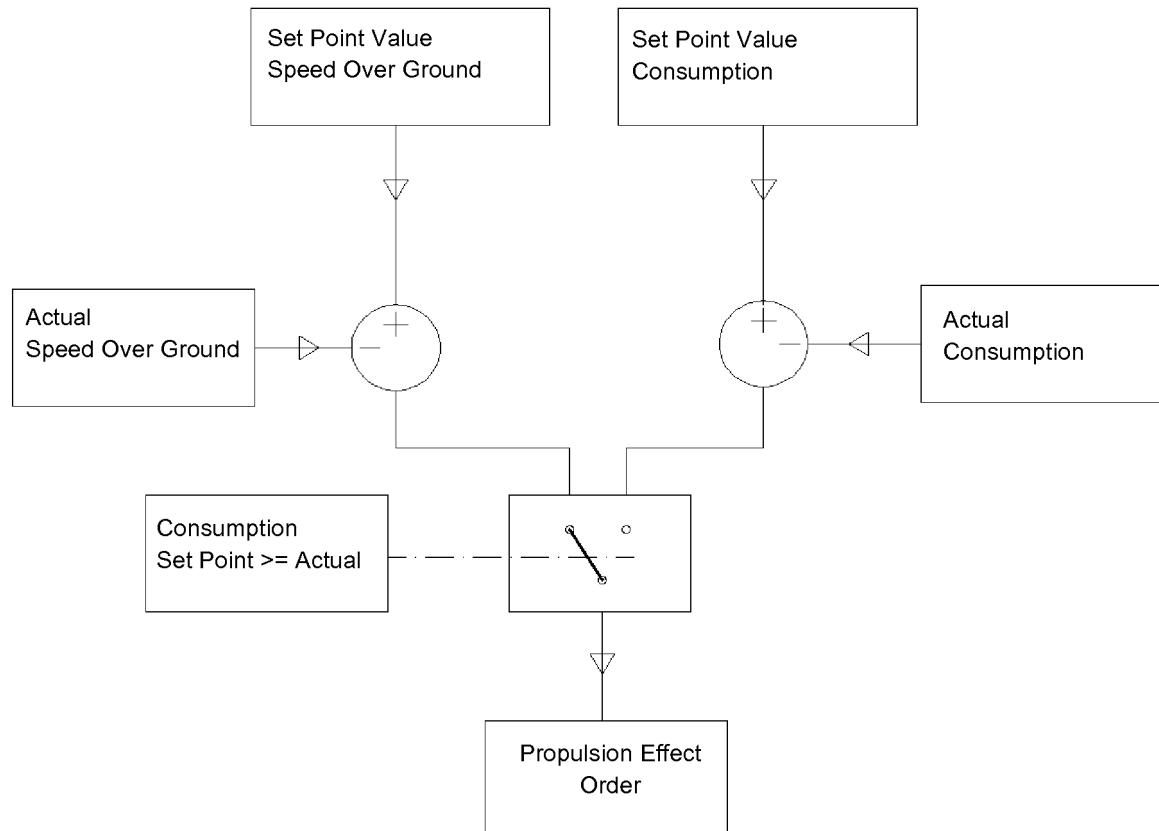
Fig. 2 Diagram of Control Logic
