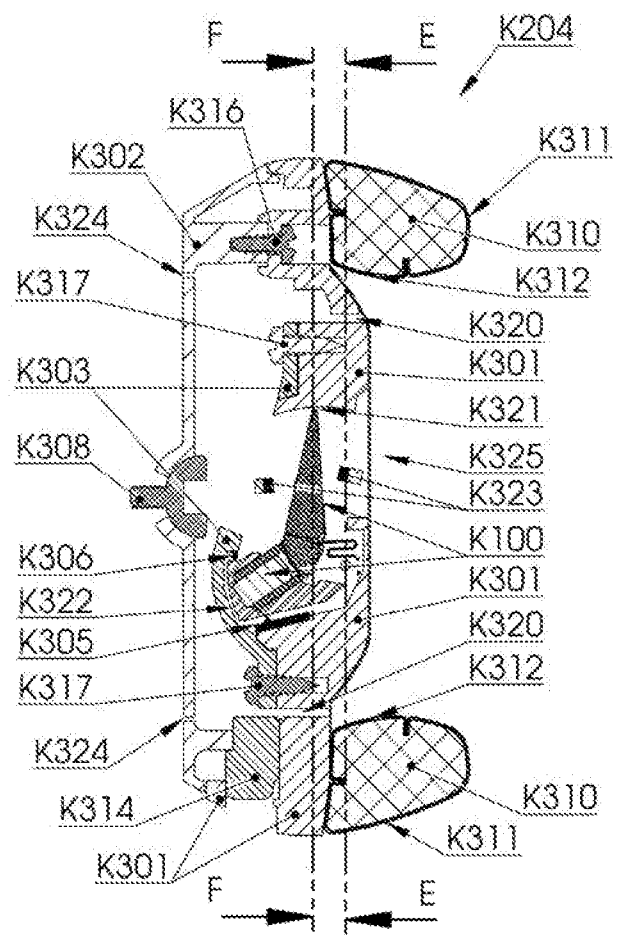
FIG. K3d SECTION D-D
