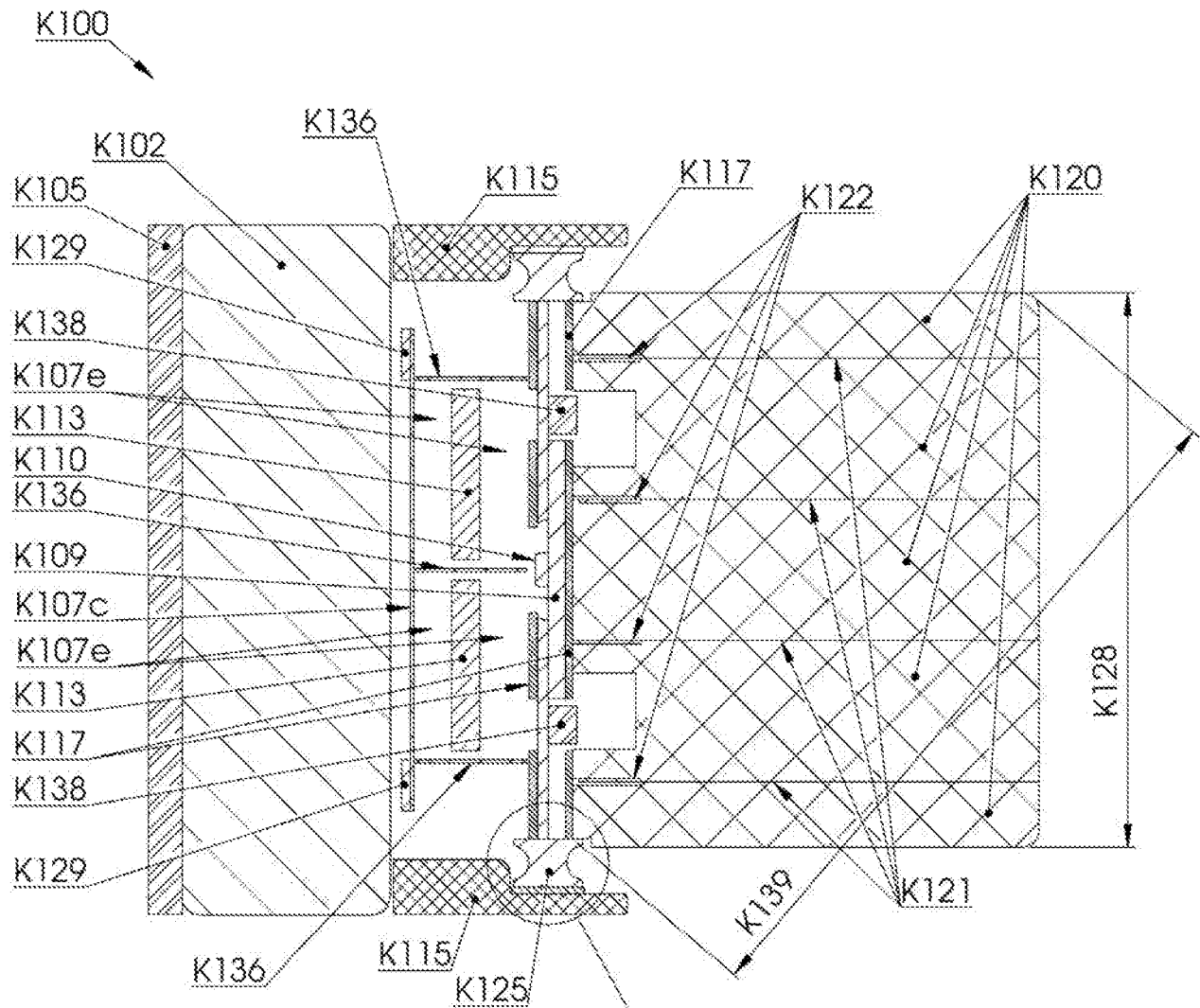
FIG. K1j SECTION B-B
