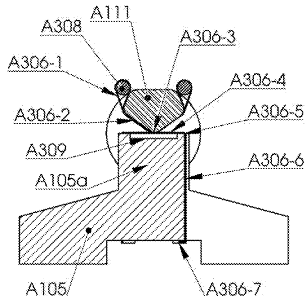
FIG. A3i SECTION C-C
