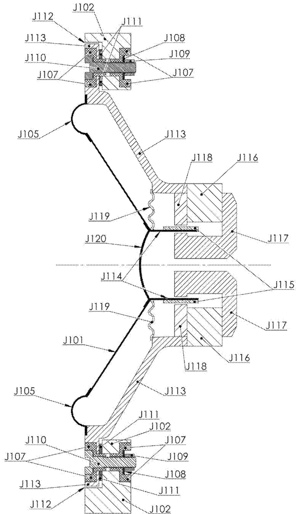
FIG. J1e PRIOR ART
