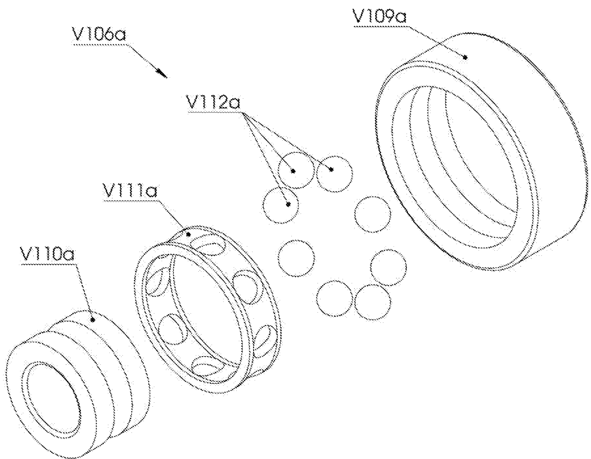
FIG. V2d (PRIOR ART)
