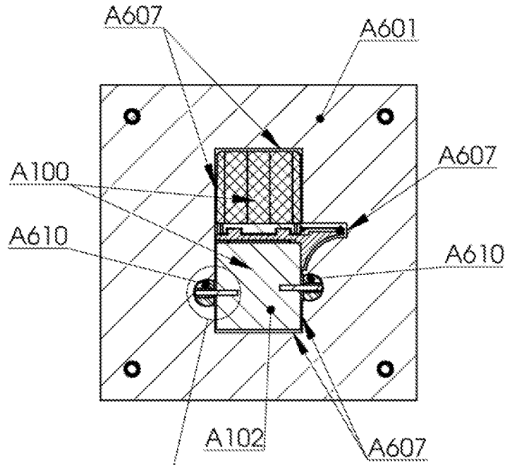
FIG. A6g SECTION B-B
