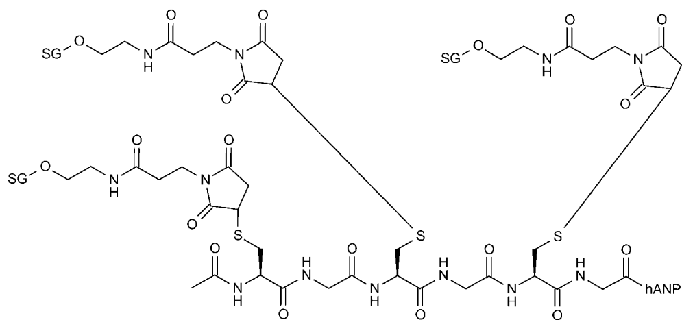
(Compound 2-15)
