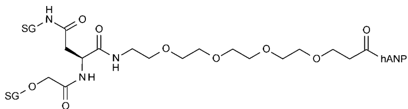
(Compound 2-13)
