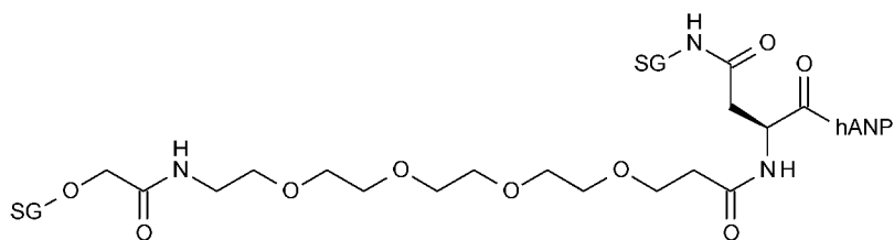
(Compound 2-16)
