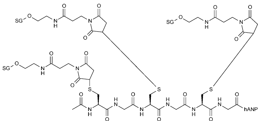
(Compound 2-15)
