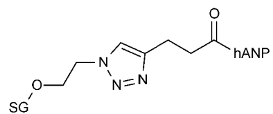
(Compound 2-12)
