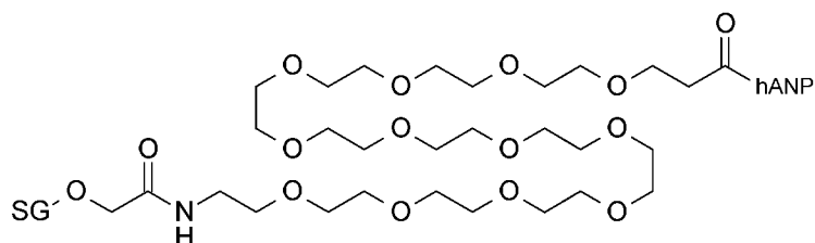
(Compound 2-30)
