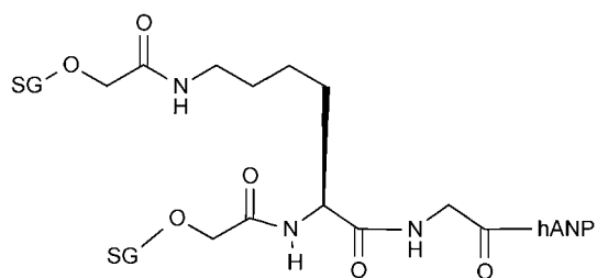
(Compound 2-14)
