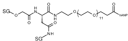
(Compound 2-27)
