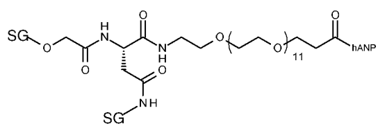
(Compound 2-27)
