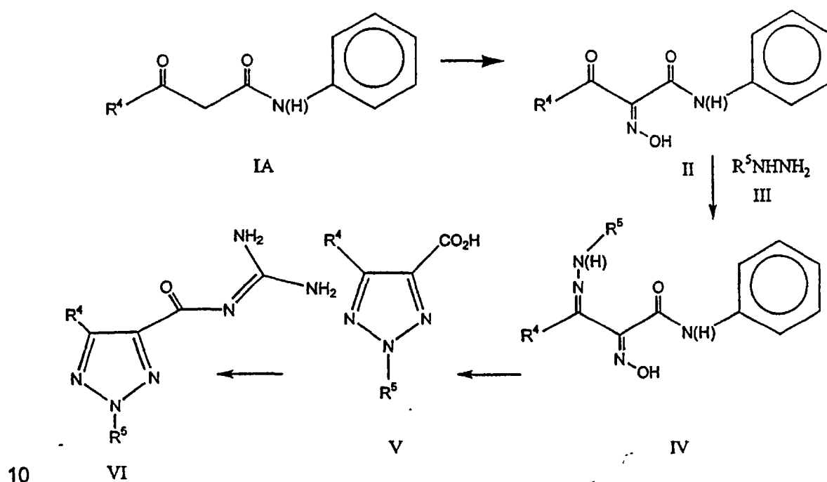
SCHEME I
