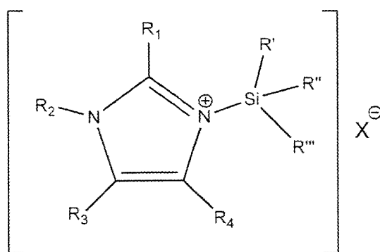
Formula I
