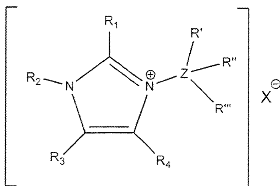
Formula II
