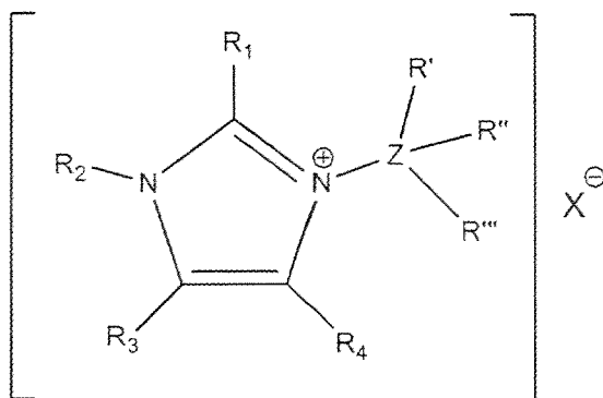
Formula II
