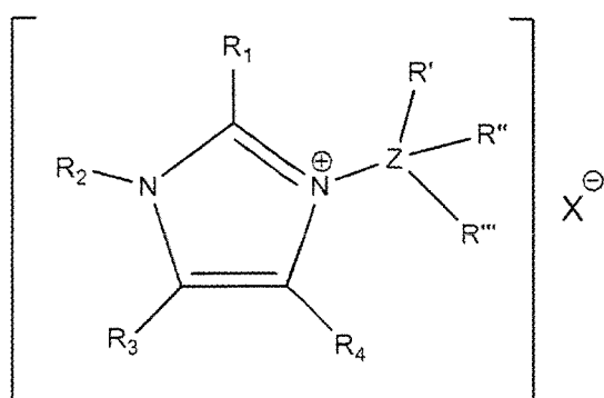
Formula II
