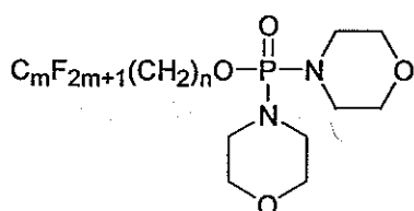
Dimorpholinophosphate
