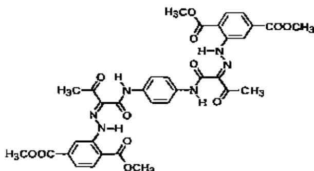
Structural Formula (3)
