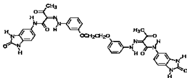
Structural Formula (2)
