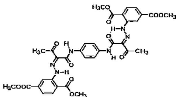
Structural Formula (3)
