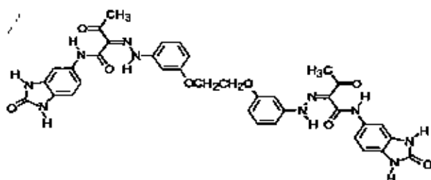
Structural Formula (2)
