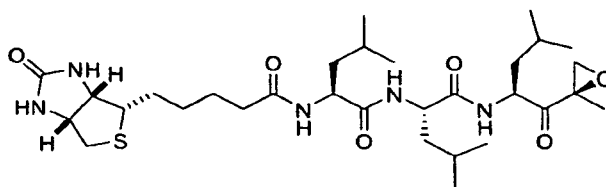
Inhibitor C
