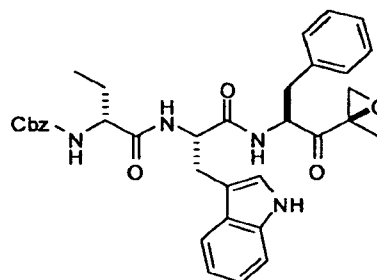
Inhibitor B
