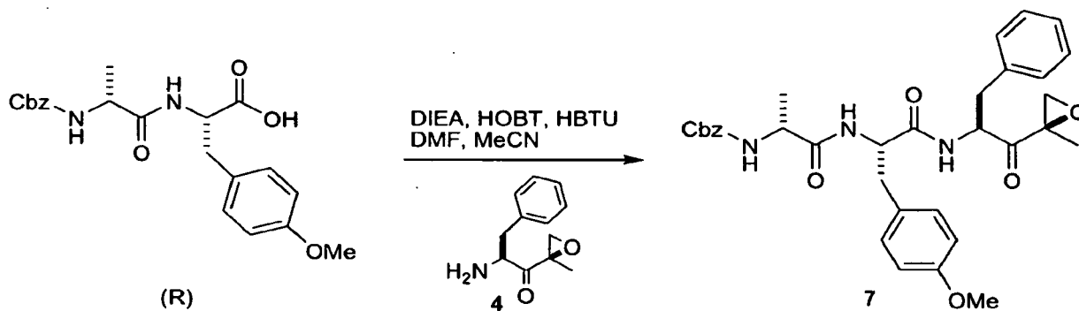
Scheme 7: Synthesis of Example 7
