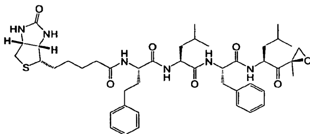
Inhibitor A
