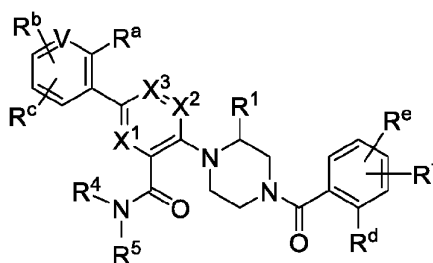
Formula (V).
