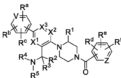
Formula (III)
