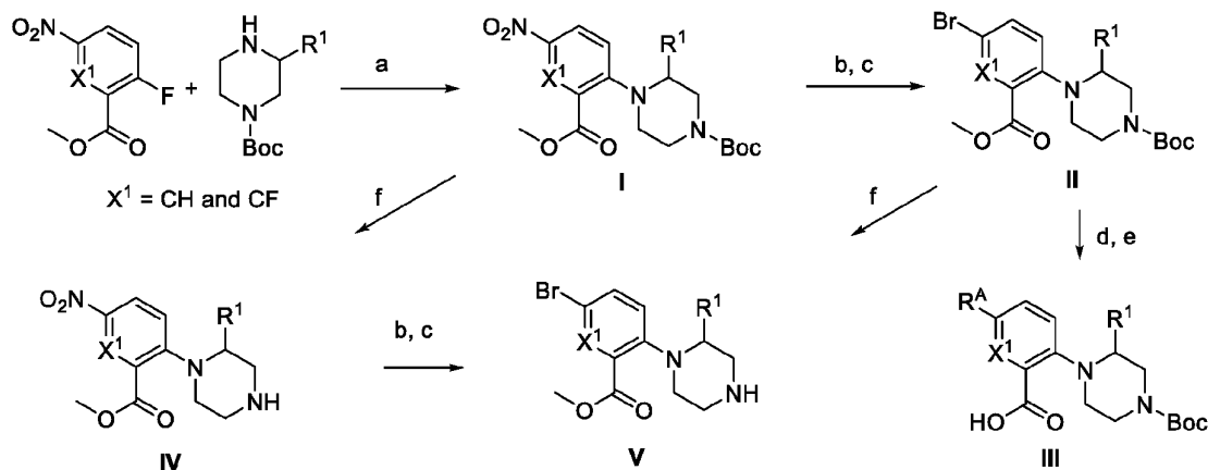
Scheme A
