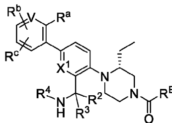
Formula (IXa)
