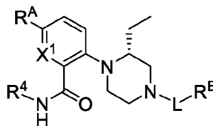
Formula (VIII).
