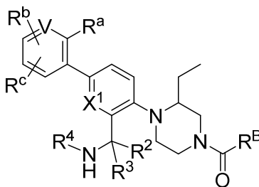
Formula (IX)
