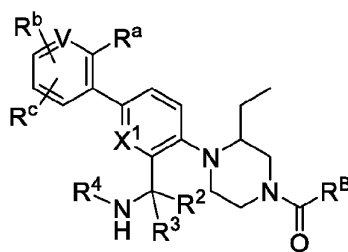
Formula (IX)
