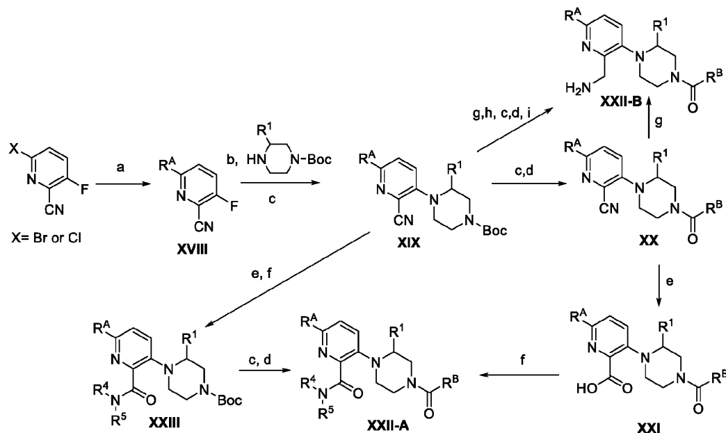
Scheme E
