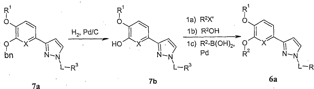
Scheme 3
