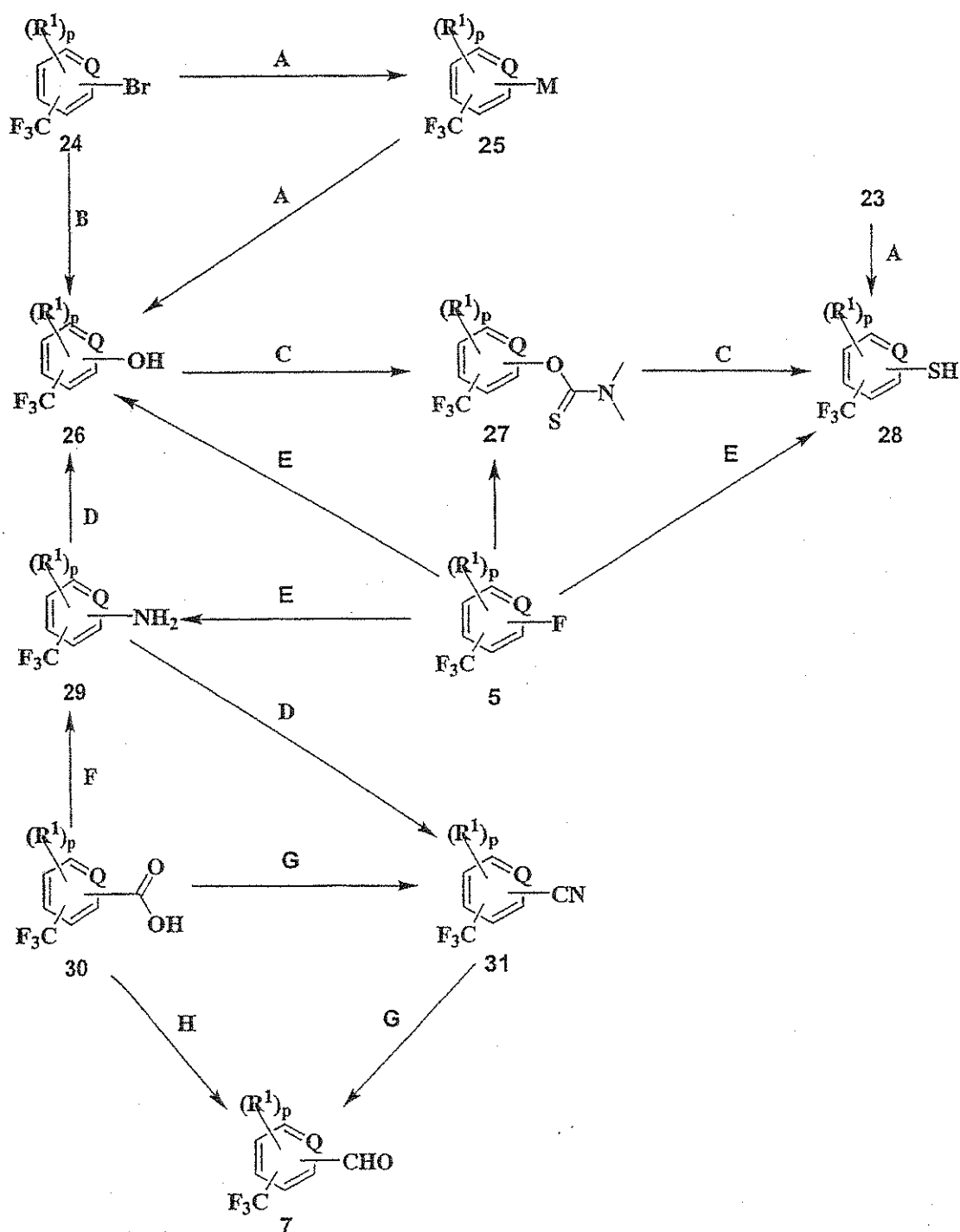
Scheme 3 - Preparations and interconversions of phenols, amines, mercaptans and aldehydes
