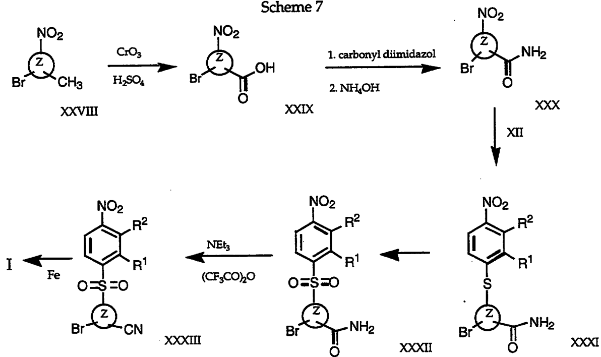
Scheme 7
