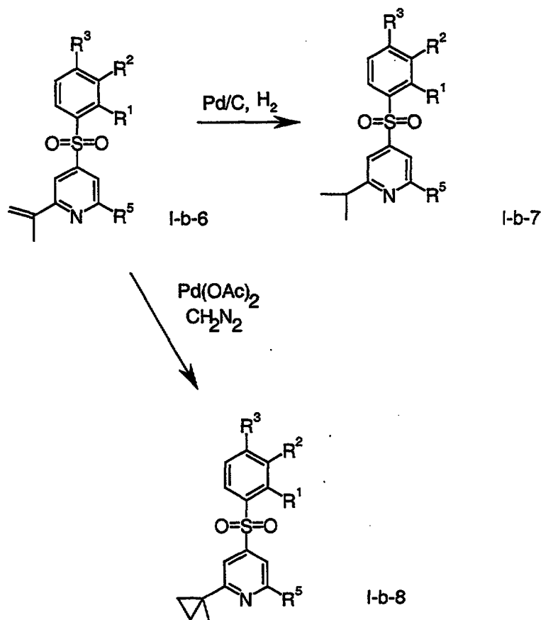
Scheme 10
