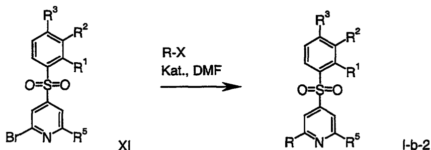
Scheme 8
