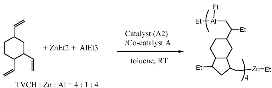
Scheme 6.
