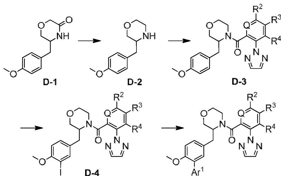
Reaction Scheme D
