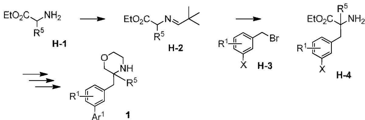
Reaction Scheme H
