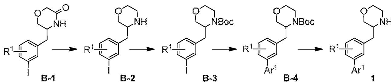
Reaction Scheme B
