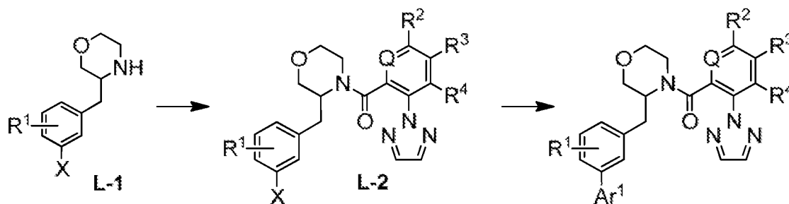
Reaction Scheme L
