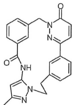
17-methyl-6,14,18,19,28-pentaazapentacyclo[20.3.1.1 2,6 .1 8,12 .0 15,19 ]octacosal(26),2(28),3,8,10,12(27),15,17,22,24-decaene-5,13-dione ( 15 )
