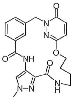
12-methyl-21-oxa-1,9,12,13,16,26-hexaazatetracyclo[20.3.1.1 3,7 .0 10,14 ]heptacos-3,5,7(27),10,13,22(26),23-heptaene-8,15,25-trione (5)
