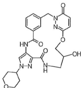
18-hydroxy-12-(oxan-4-yl)-20-oxa-1,9,12,13,16,25-hexaazatetracyclo[19.3.1.1 3,7 .0 10,14 ]hexacosa-3,5,7(26),10,13,21(25),22-heptaene-8,15,24-trione (11)
