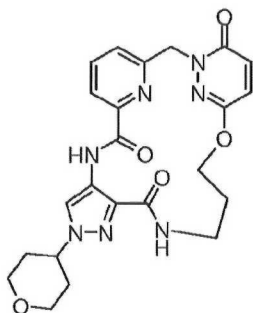
12-(oxan-4-yl)-20-oxa-1,9,12,13,16,25,26-heptaazatetracyclo[19.3.1.1 3,7 .0 10,14 ]hexacos-3,5,7(26),10,13,21(25),22-heptaene-8,15,24-trione (9)
