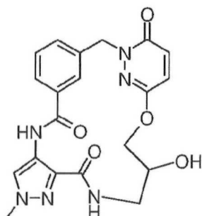
18-hydroxy-12-methyl-20-oxa-1,9,12,13,16,25-hexaazatetracyclo[19.3.1.1 3,7 .0 10,14 ]hexacos-3,5,7(26),10,13,21(25),22-heptaene-8,15,24-trione (12)
