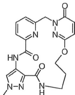
12-methyl-20-oxa-1,9,12,13,16,25,26-heptaazatetracyclo[19.3.1.1 3,7 .0 10,14 ]hexacos-3,5,7(26),10,13,21(25),22-heptaene-8,15,24-trione (8)
