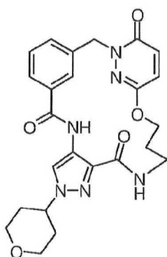
12-(oxan-4-yl)-20-oxa-1,9,12,13,16,25-hexaazatetracyclo[19.3.1.1 3,7 .0 10,14 ]hexacos-3,5,7(26),10,13,21(25),22-heptaene-8,15,24-trione (6)
