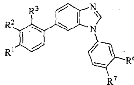
Formula VIIa
