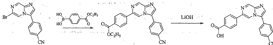
Intermediate 11
