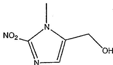
N-1-methyl-2-nitro-5-hydroxymethyl imidazole
